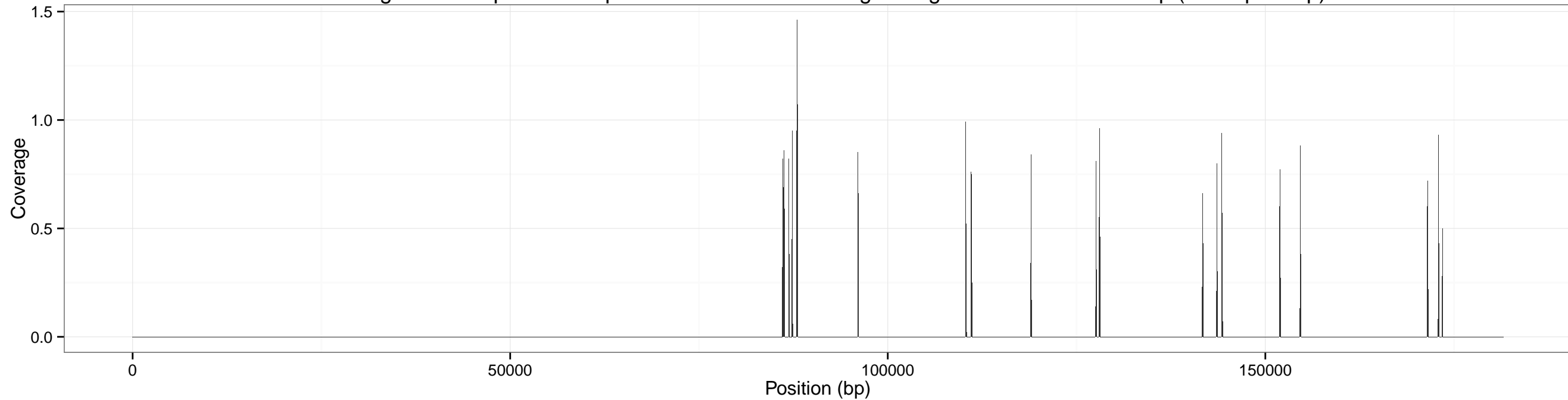
Coverage accross pXO1 for input SRR1749070-0x using sliding window of size: 100 bp (overlap 50 bp)
