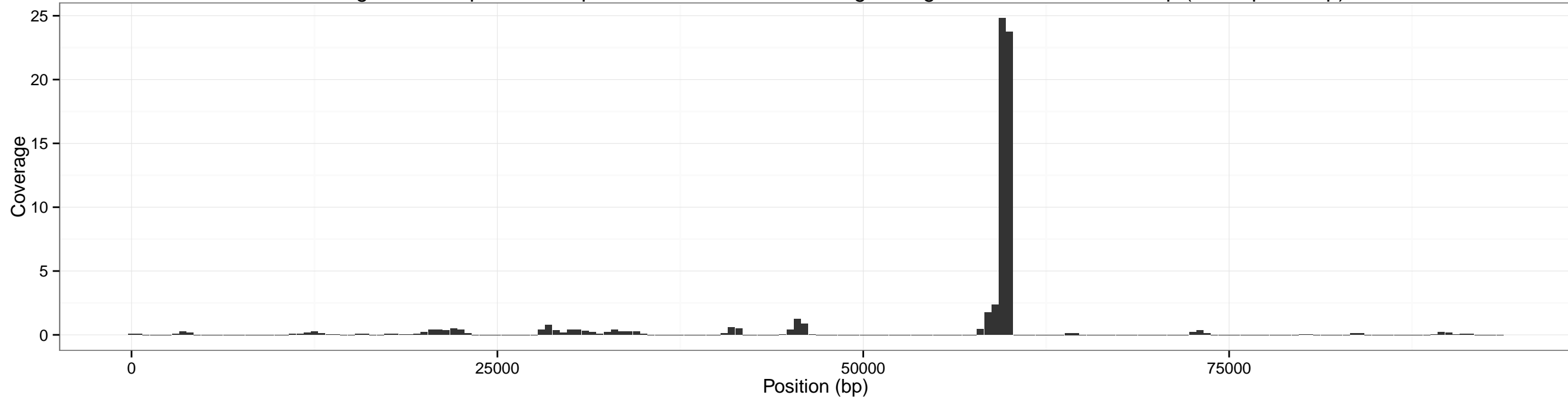
Coverage across pXO2 for input SRR1749070-0.5x using sliding window of size: 1000 bp (overlap 500 bp)
