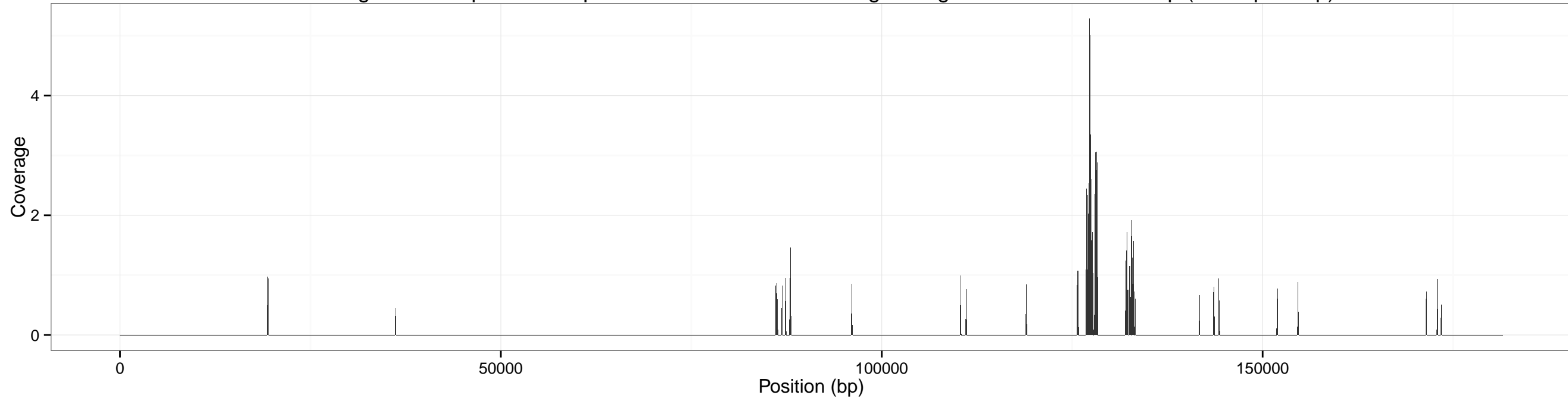
Coverage accross pXO1 for input SRR1749070-0.25x using sliding window of size: 100 bp (overlap 50 bp)
