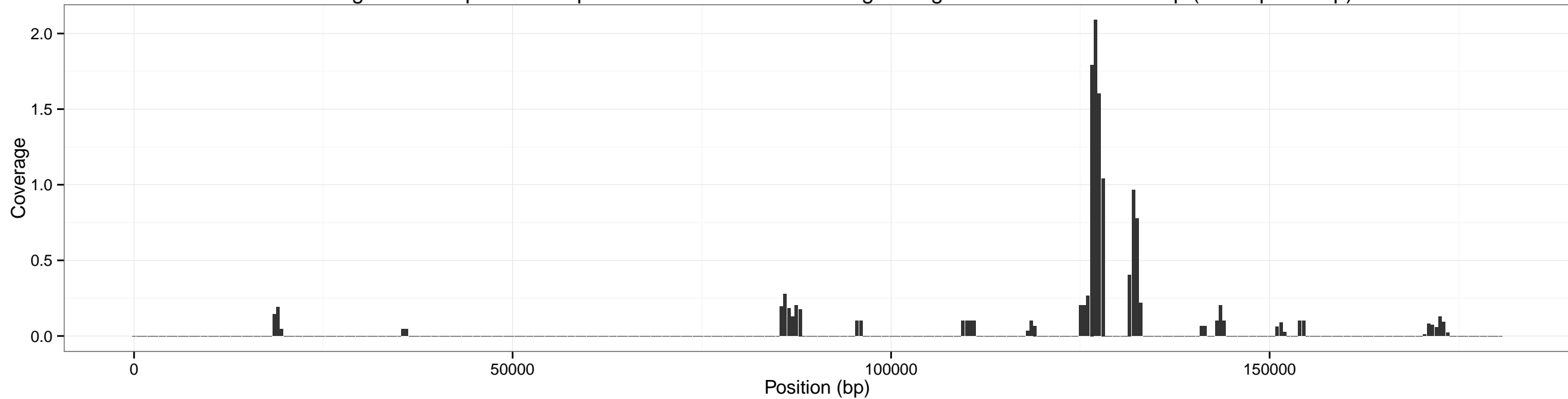
Coverage accross pXO1 for input SRR1749070-0.25x using sliding window of size: 1000 bp (overlap 500 bp)
