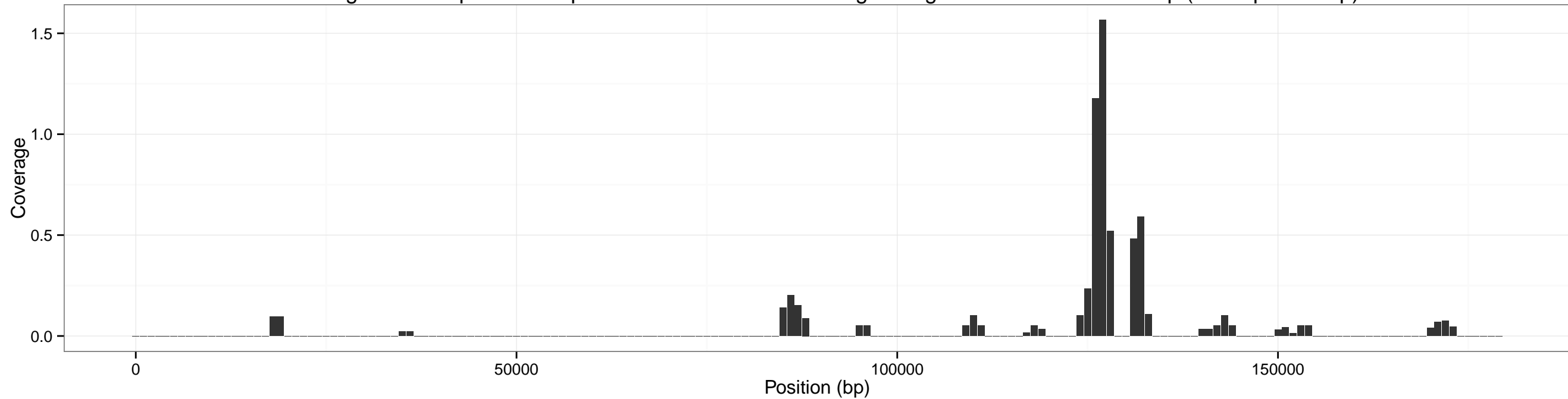
Coverage across pXO1 for input SRR1749070-0.25x using sliding window of size: 2000 bp (overlap 1000 bp)
