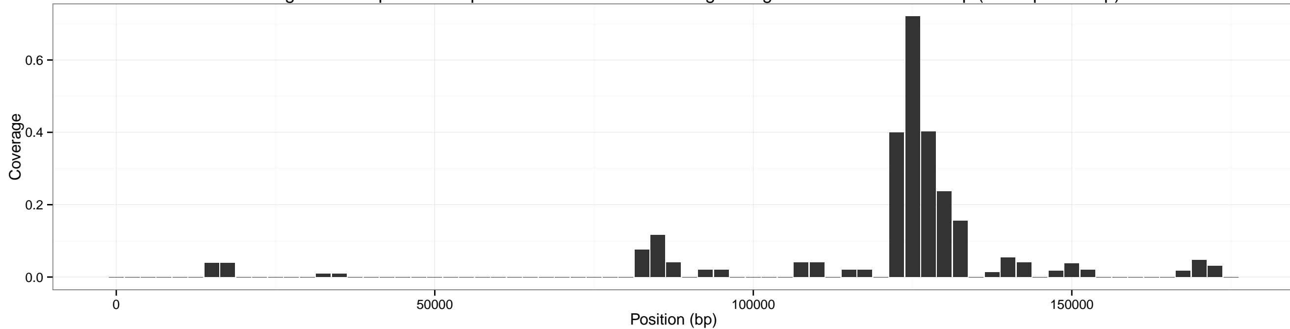
Coverage across pXO1 for input SRR1749070-0.25x using sliding window of size: 5000 bp (overlap 2500 bp)
