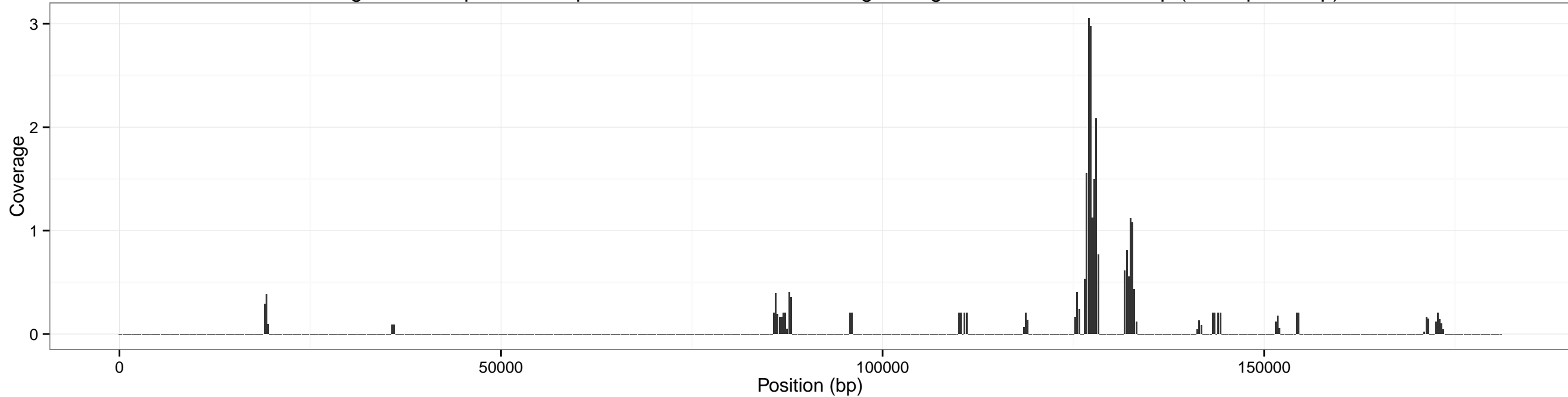
Coverage accross pXO1 for input SRR1749070-0.25x using sliding window of size: 500 bp (overlap 250 bp)
