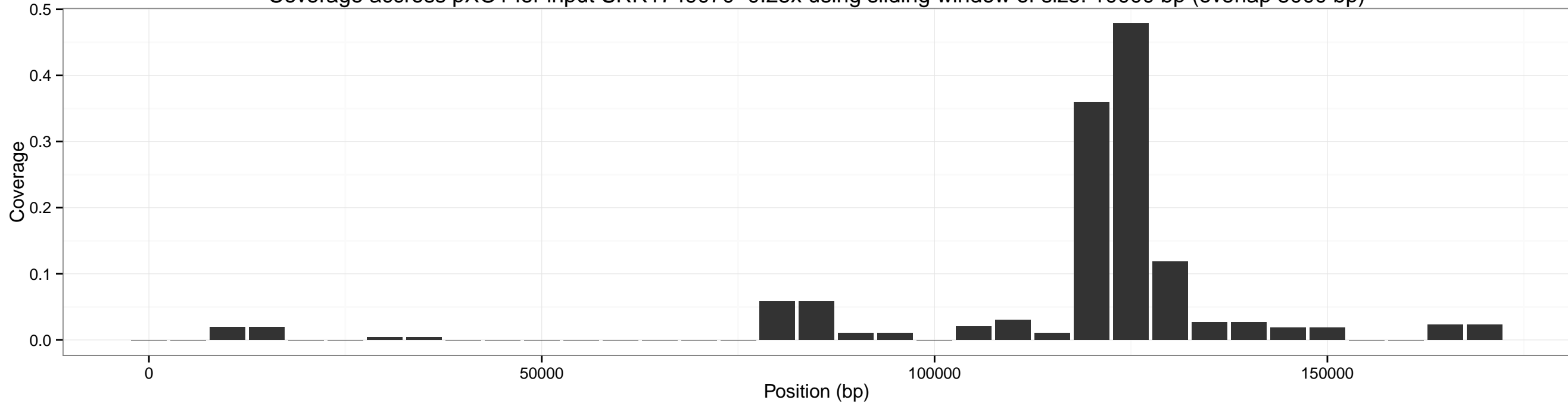
Coverage across pXO1 for input SRR1749070-0.25x using sliding window of size: 10000 bp (overlap 5000 bp)
