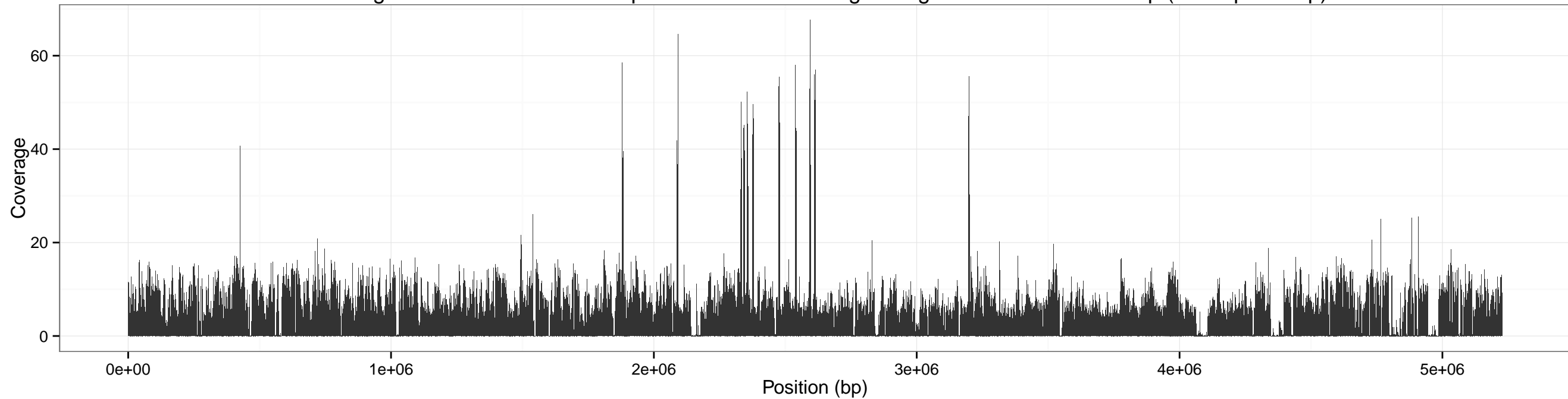
Coverage accross anthracis for input SRR1749083 using sliding window of size: 500 bp (overlap 250 bp)
