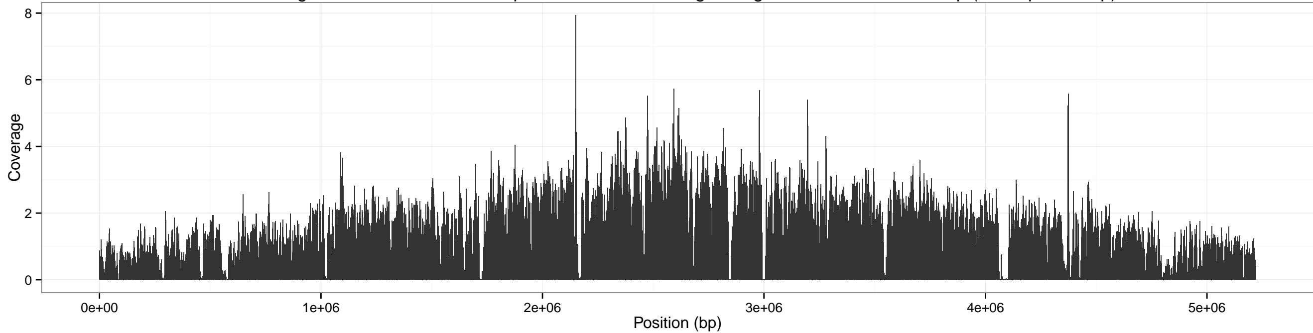
Coverage accross anthracis for input SRR1748707 using sliding window of size: 5000 bp (overlap 2500 bp)
