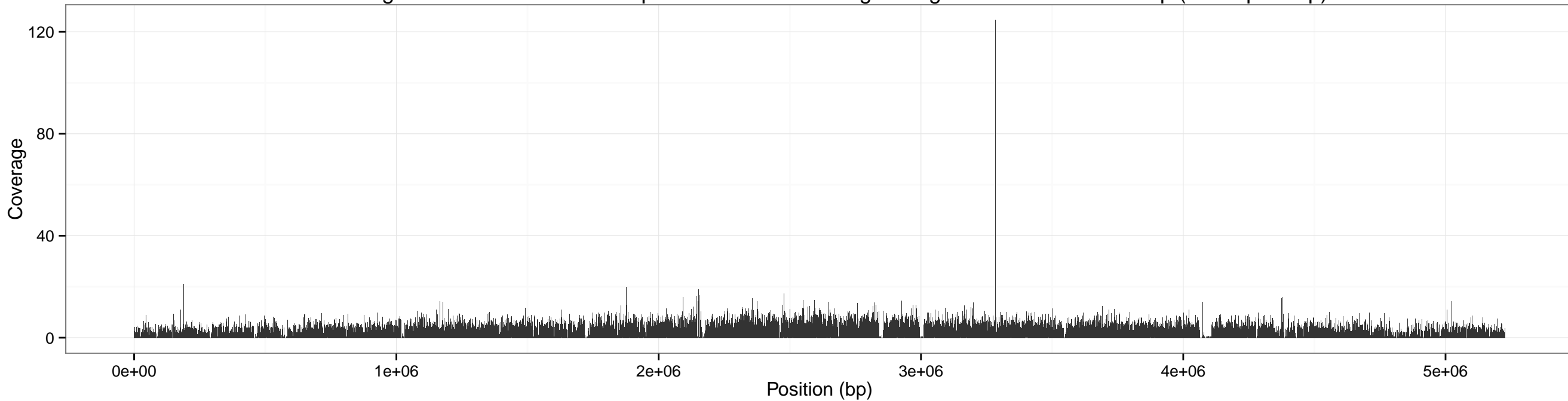
Coverage accross anthracis for input SRR1748707 using sliding window of size: 100 bp (overlap 50 bp)
