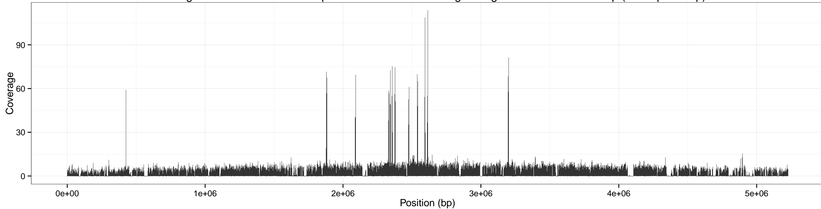
Coverage accross anthracis for input SRR1749070-5x using sliding window of size: 500 bp (overlap 250 bp)
