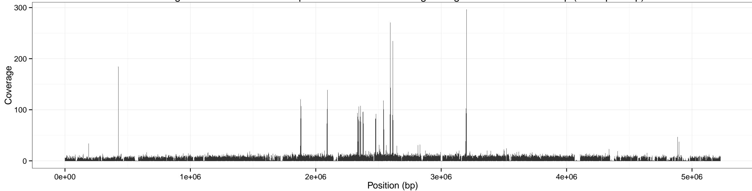
Coverage across anthracis for input SRR1749070-5x using sliding window of size: 100 bp (overlap 50 bp)
