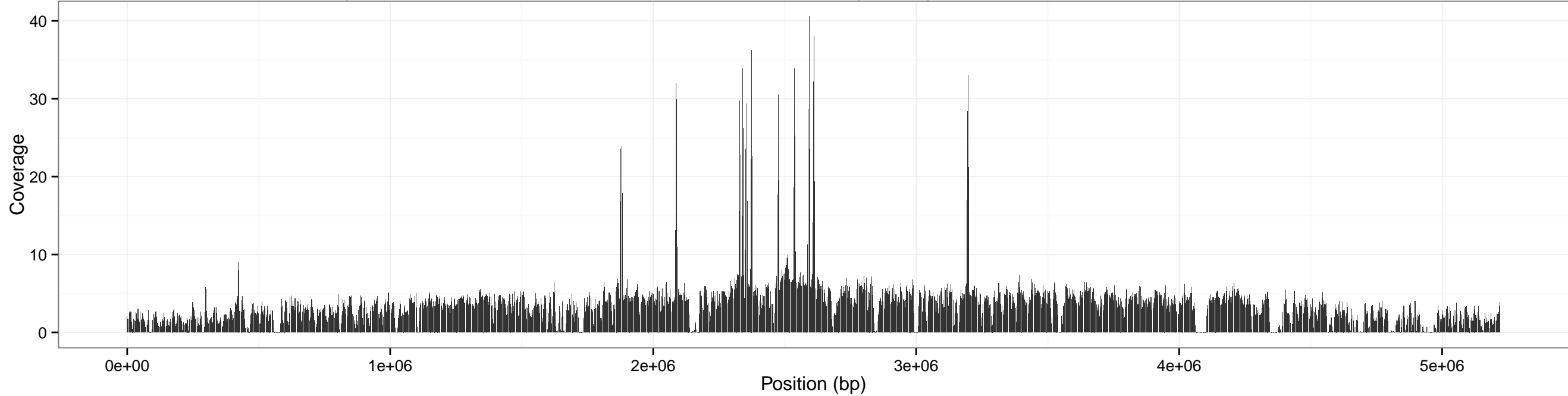
Coverage across anthracis for input SRR1749070-5x using sliding window of size: 5000 bp (overlap 2500 bp)
