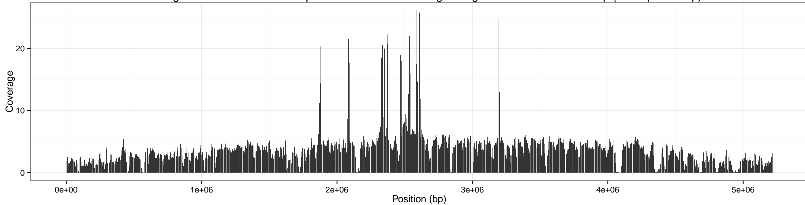
Coverage across anthracis for input SRR1749070-5x using sliding window of size: 10000 bp (overlap 5000 bp)
