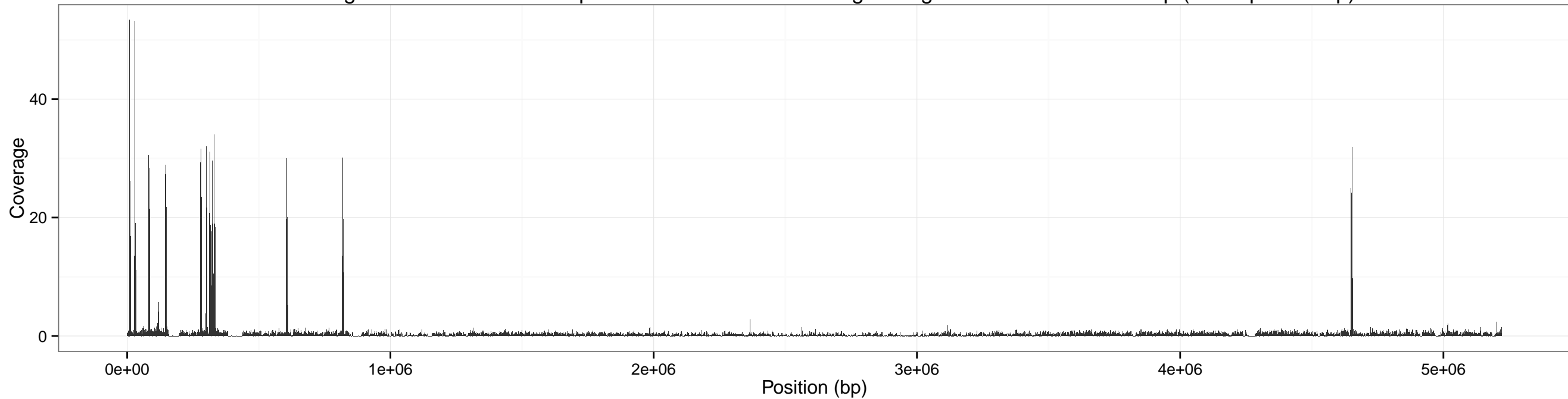
Coverage accross cereus for input SRR1749070-0.5x using sliding window of size: 2000 bp (overlap 1000 bp)
