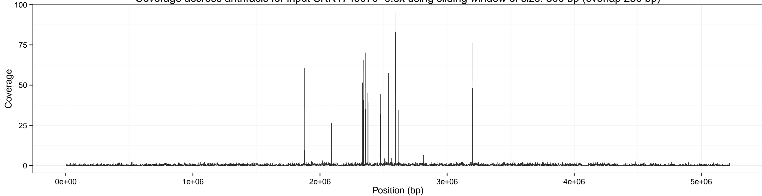
Coverage across anthracis for input SRR1749070-0.5x using sliding window of size: 500 bp (overlap 250 bp)
