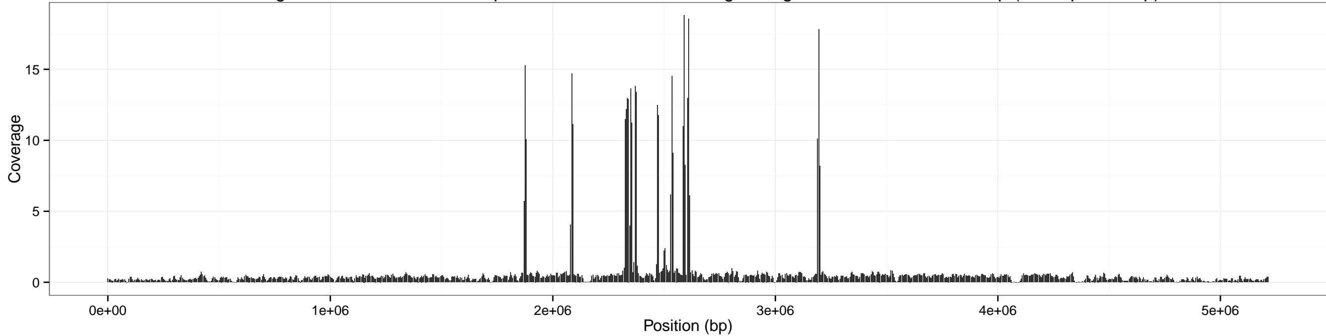
Coverage across anthracis for input SRR1749070-0.5x using sliding window of size: 10000 bp (overlap 5000 bp)
