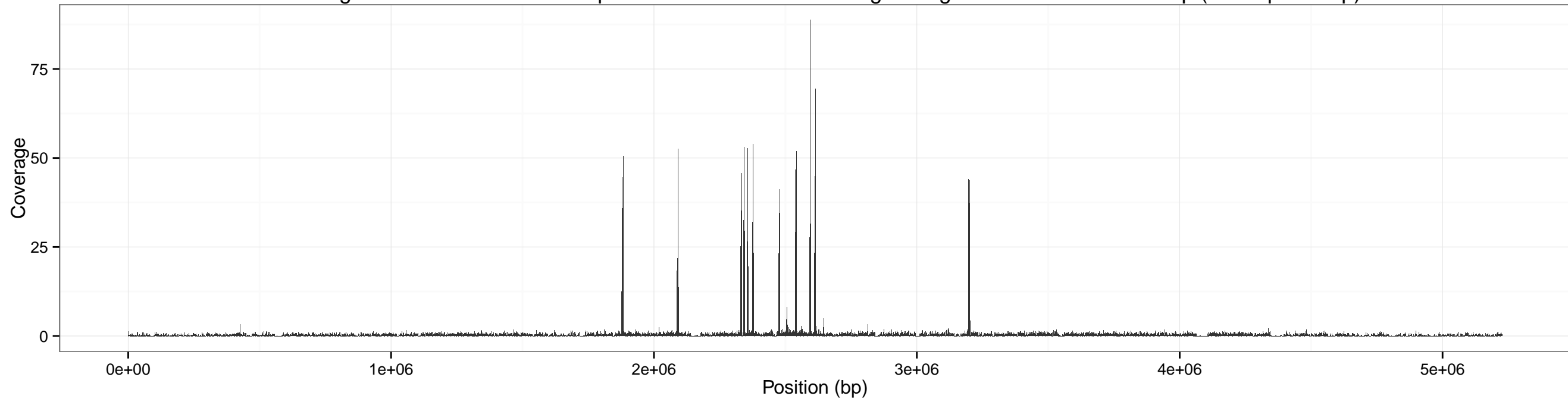
Coverage across anthracis for input SRR1749070-0.5x using sliding window of size: 1000 bp (overlap 500 bp)
