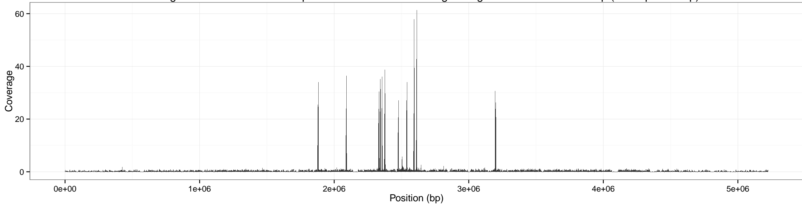
Coverage across anthracis for input SRR1749070-0.5x using sliding window of size: 2000 bp (overlap 1000 bp)
