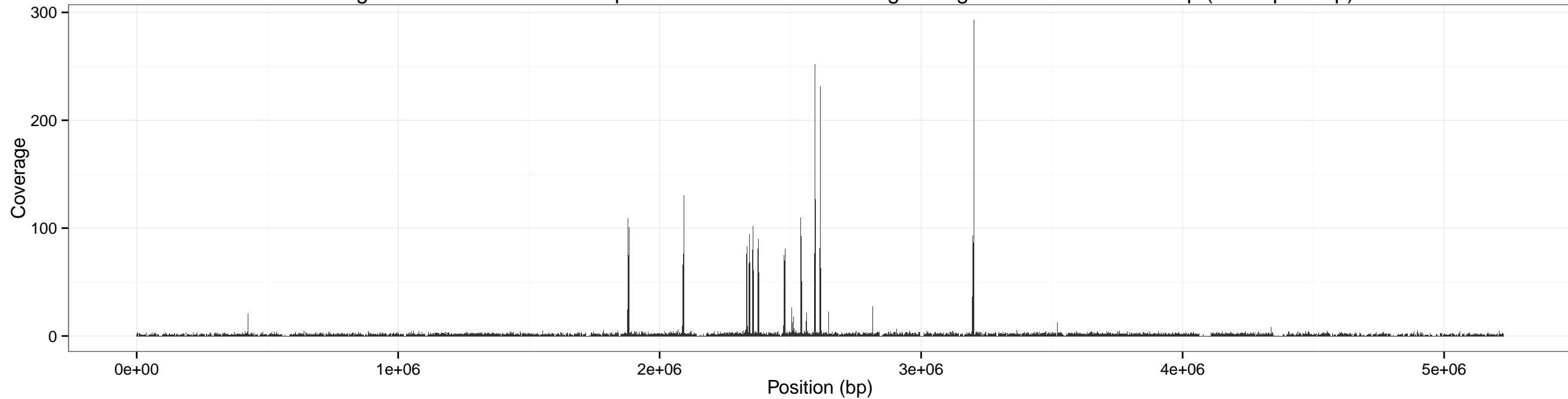
Coverage across anthracis for input SRR1749070-0.5x using sliding window of size: 100 bp (overlap 50 bp)
