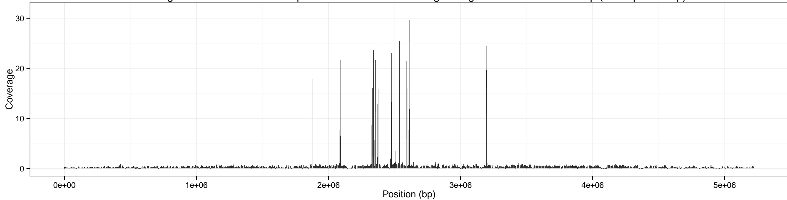
Coverage across anthracis for input SRR1749070-0.5x using sliding window of size: 5000 bp (overlap 2500 bp)
