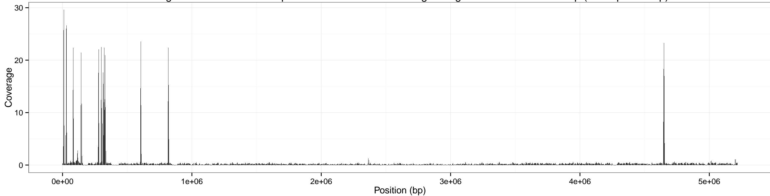
Coverage across cereus for input SRR1749070-0.25x using sliding window of size: 5000 bp (overlap 2500 bp)
