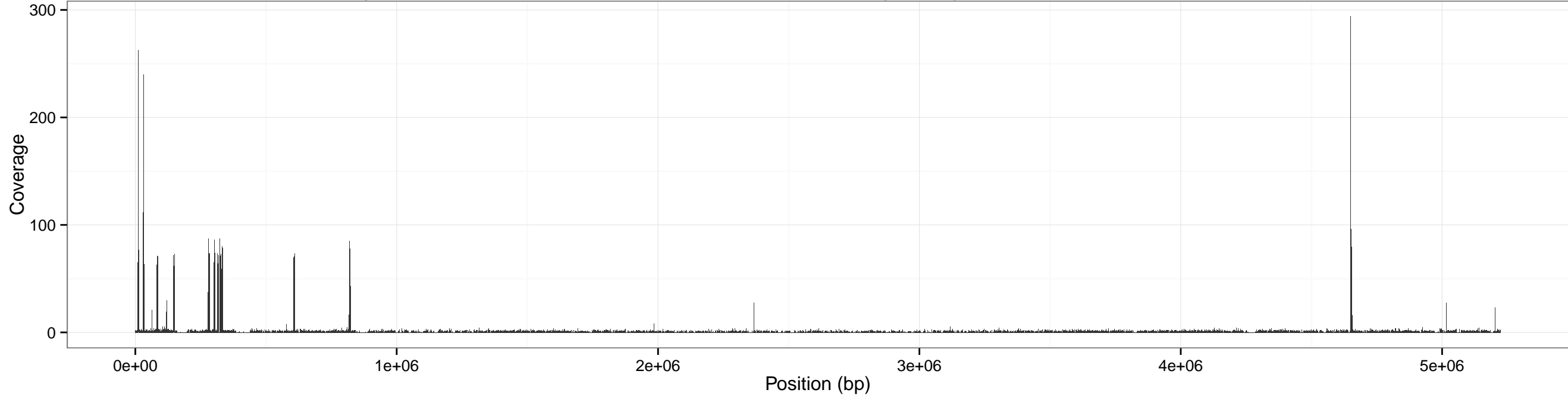
Coverage across cereus for input SRR1749070-0.25x using sliding window of size: 100 bp (overlap 50 bp)
