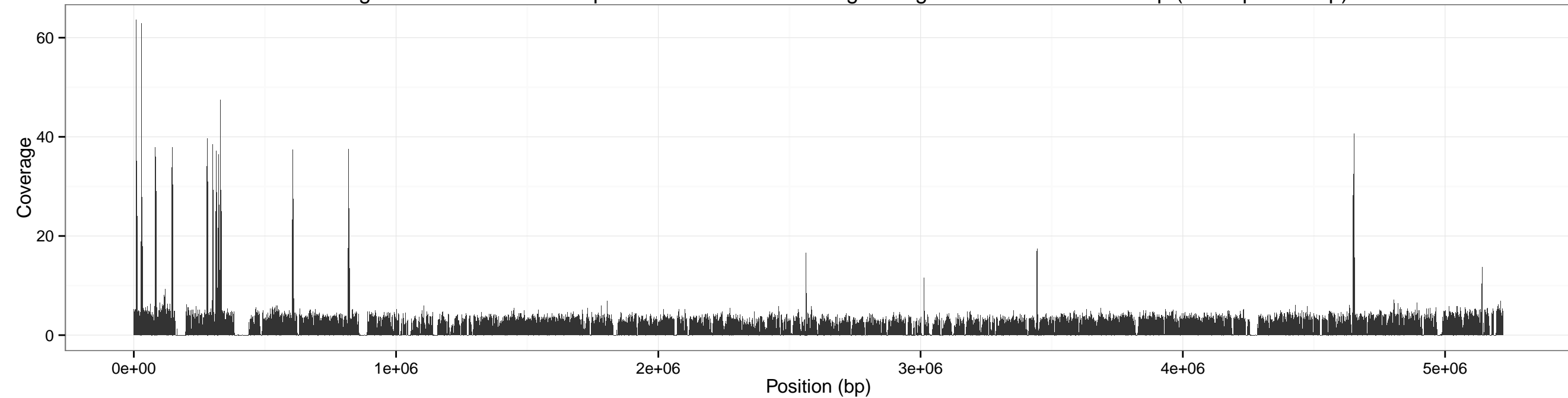
Coverage across cereus for input SRR1749070-5x using sliding window of size: 2000 bp (overlap 1000 bp)
