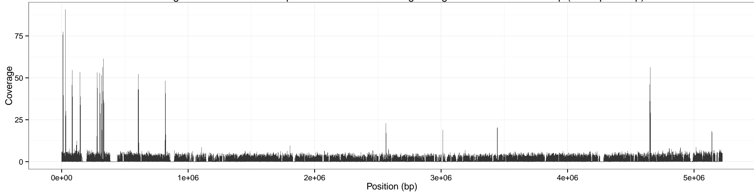
Coverage across cereus for input SRR1749070-5x using sliding window of size: 1000 bp (overlap 500 bp)
