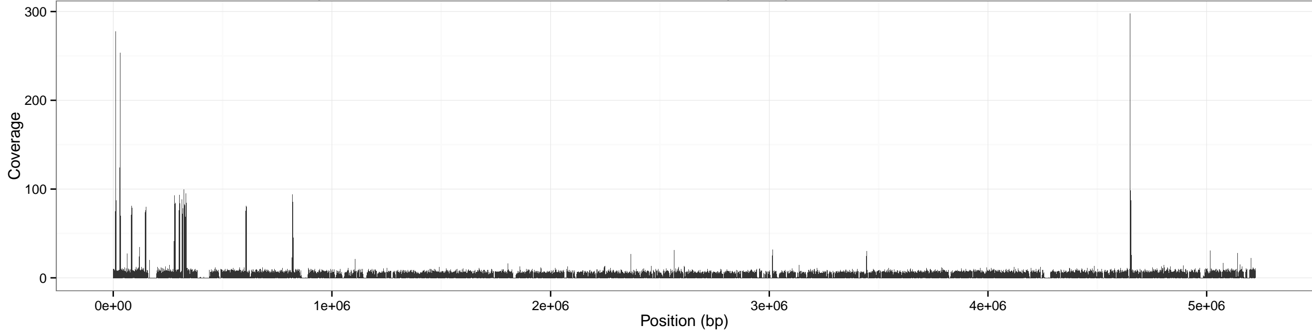
Coverage accross cereus for input SRR1749070-5x using sliding window of size: 100 bp (overlap 50 bp)
