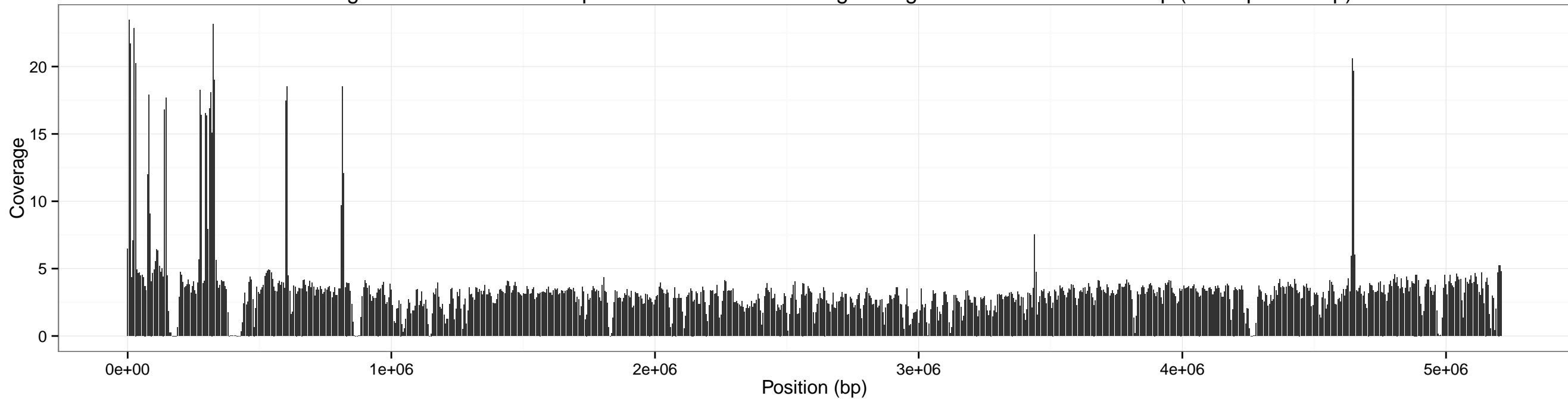
Coverage across cereus for input SRR1749070-5x using sliding window of size: 10000 bp (overlap 5000 bp)
