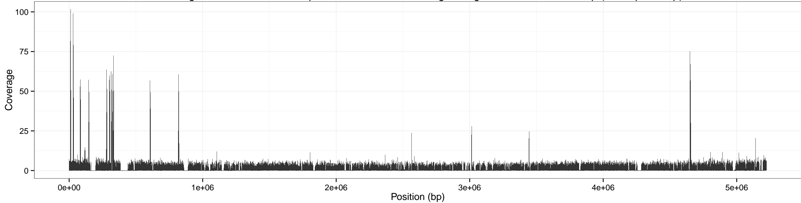
Coverage accross cereus for input SRR1749070-5x using sliding window of size: 500 bp (overlap 250 bp)
