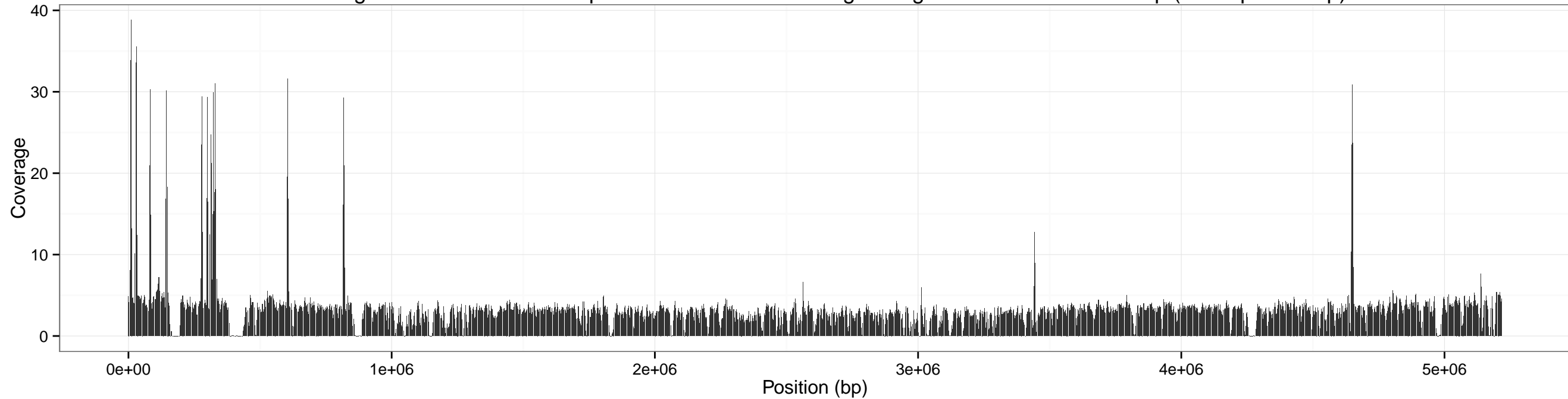
Coverage accross cereus for input SRR1749070-5x using sliding window of size: 5000 bp (overlap 2500 bp)
