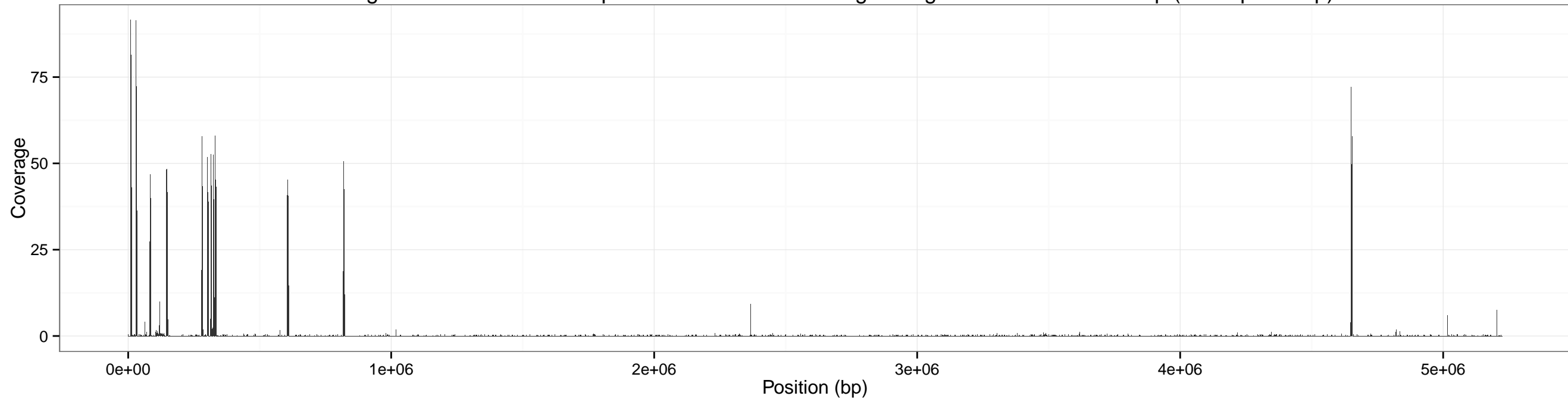
Coverage accross cereus for input SRR1749070-0x using sliding window of size: 500 bp (overlap 250 bp)
