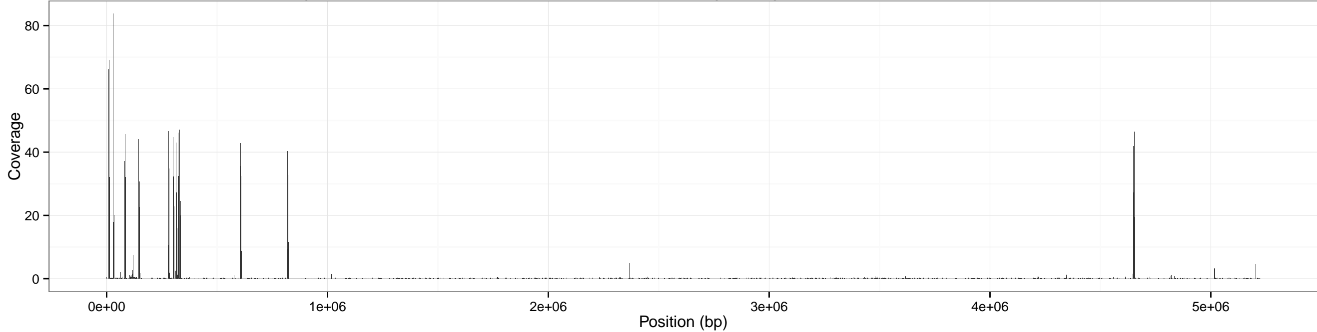
Coverage across cereus for input SRR1749070-0x using sliding window of size: 1000 bp (overlap 500 bp)
