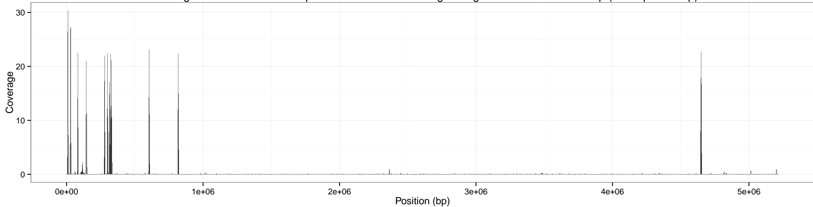
Coverage accross cereus for input SRR1749070-0x using sliding window of size: 5000 bp (overlap 2500 bp)
