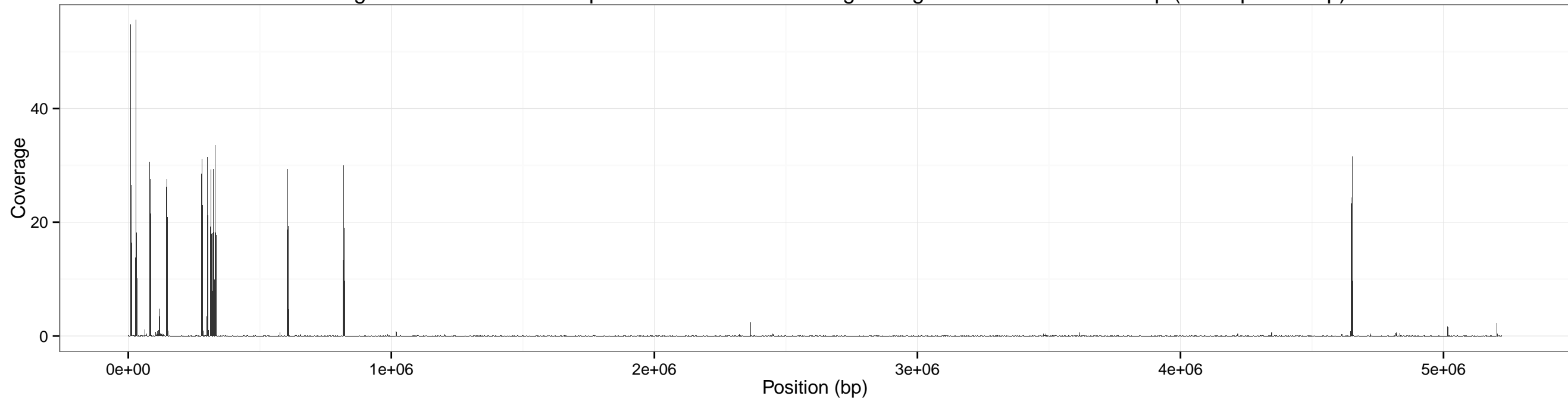
Coverage accross cereus for input SRR1749070-0x using sliding window of size: 2000 bp (overlap 1000 bp)
