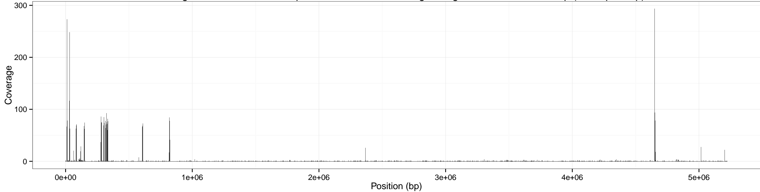
Coverage accross cereus for input SRR1749070-0x using sliding window of size: 100 bp (overlap 50 bp)
