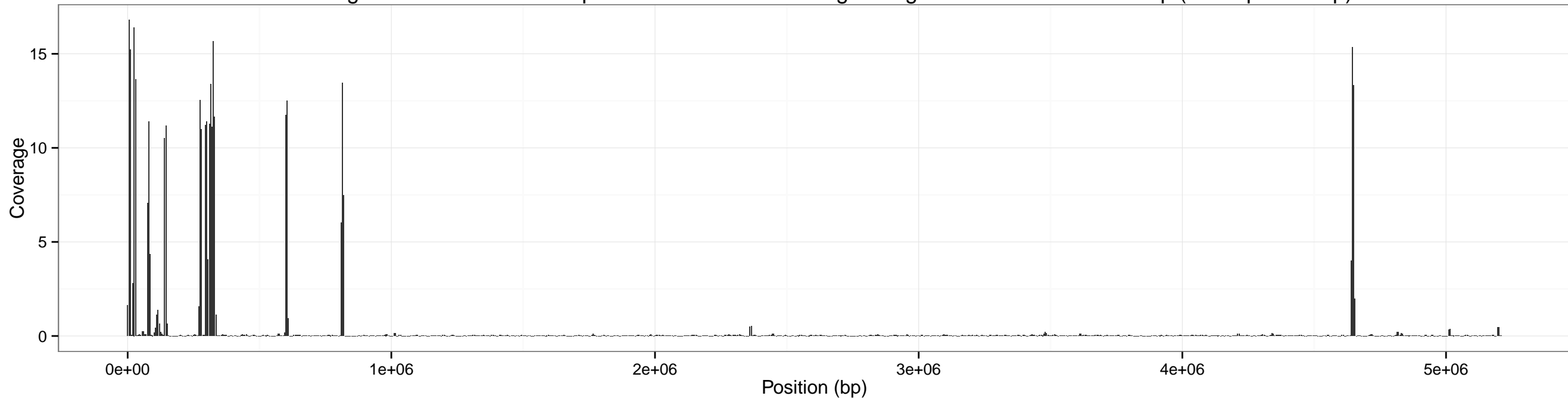
Coverage across cereus for input SRR1749070-0x using sliding window of size: 10000 bp (overlap 5000 bp)
