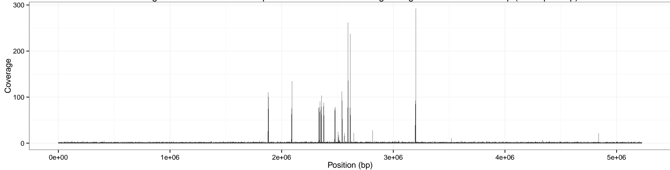
Coverage accross anthracis for input SRR1749070-0.5x using sliding window of size: 100 bp (overlap 50 bp)
