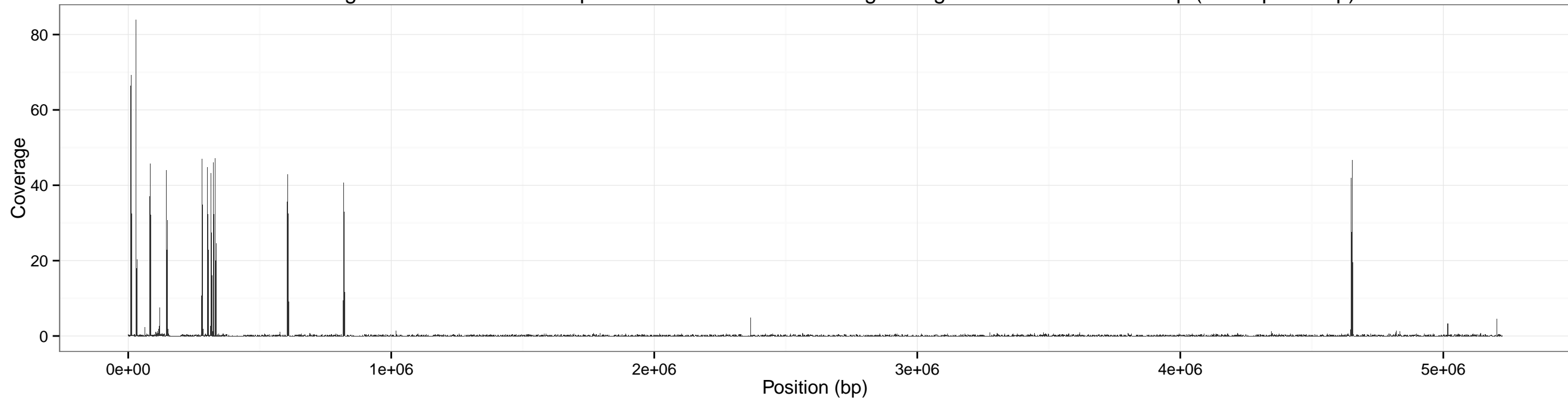
Coverage accross cereus for input SRR1749070-0.10x using sliding window of size: 1000 bp (overlap 500 bp)
