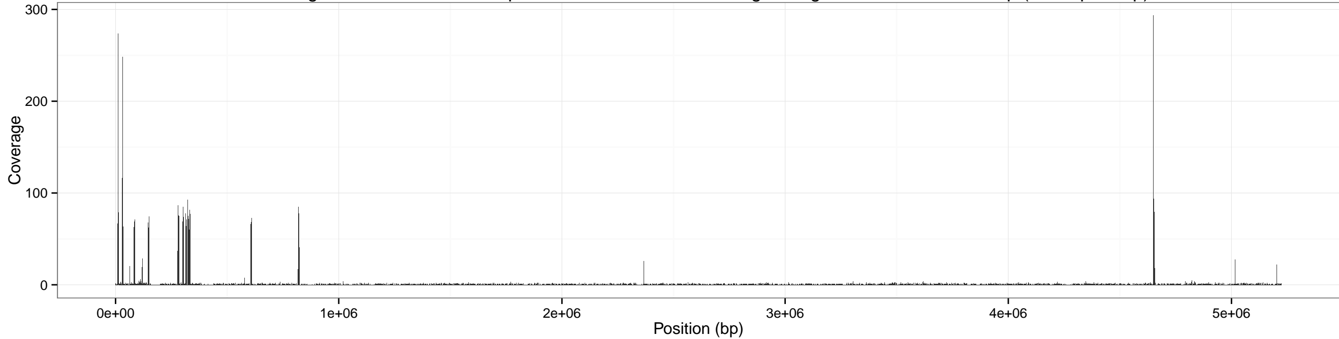
Coverage across cereus for input SRR1749070-0.10x using sliding window of size: 100 bp (overlap 50 bp)
