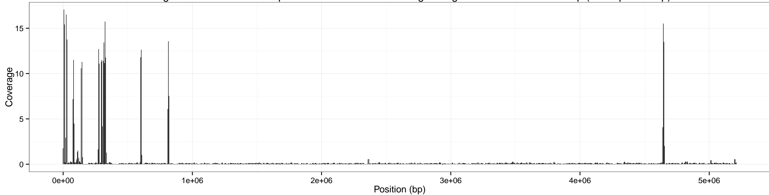
Coverage across cereus for input SRR1749070-0.10x using sliding window of size: 10000 bp (overlap 5000 bp)
