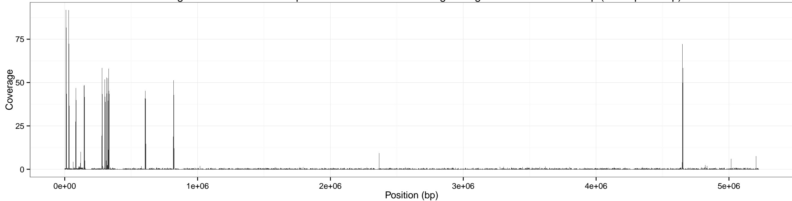
Coverage across cereus for input SRR1749070-0.10x using sliding window of size: 500 bp (overlap 250 bp)
