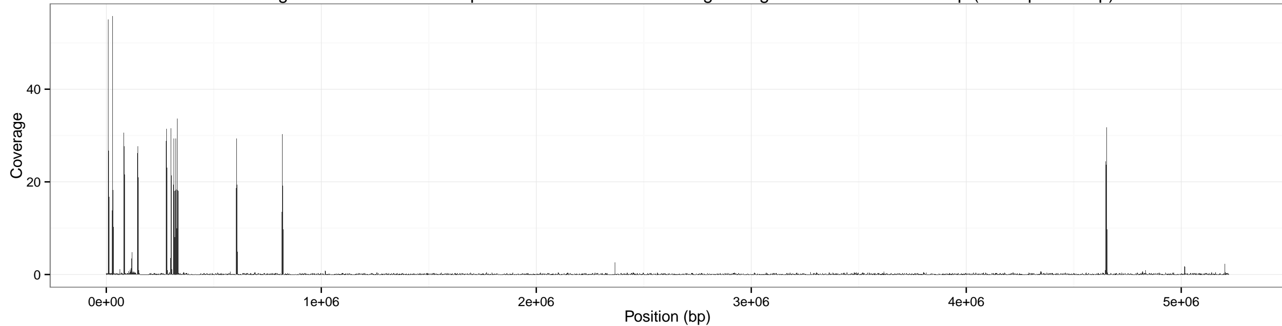
Coverage accross cereus for input SRR1749070-0.10x using sliding window of size: 2000 bp (overlap 1000 bp)
