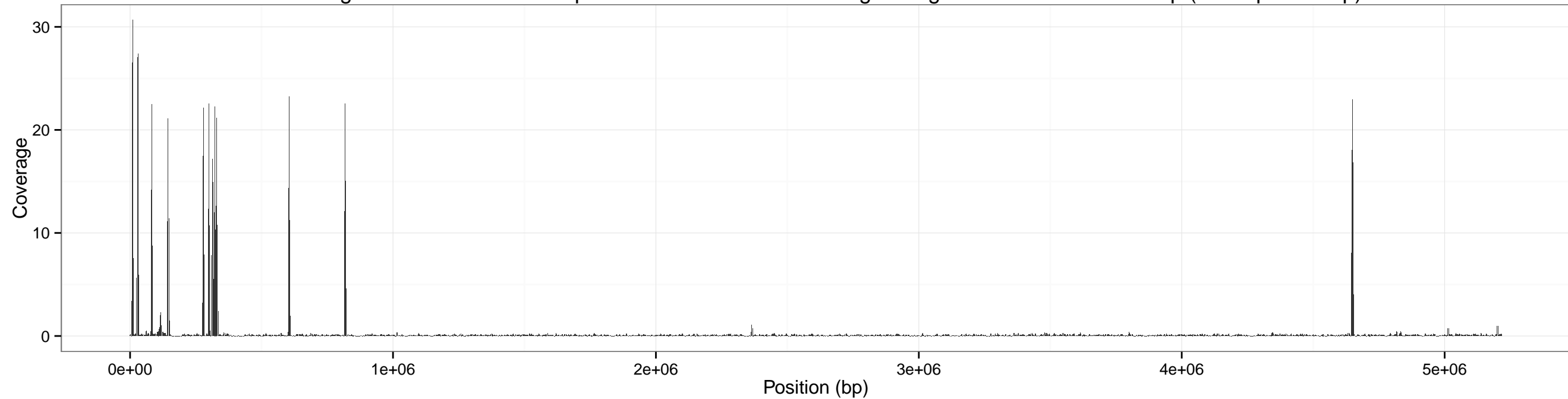
Coverage accross cereus for input SRR1749070-0.10x using sliding window of size: 5000 bp (overlap 2500 bp)
