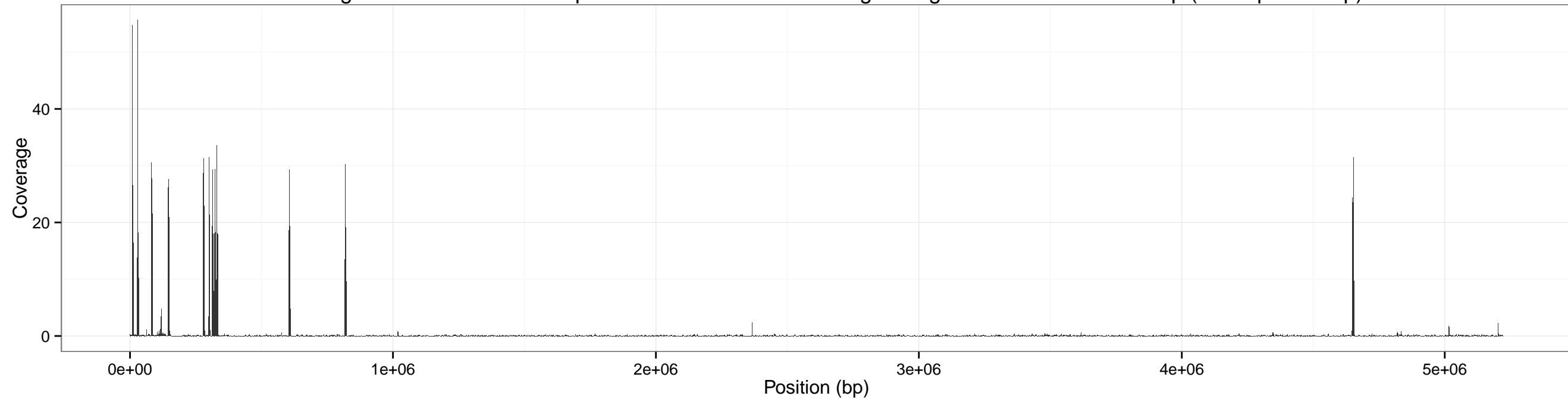
Coverage across cereus for input SRR1749070-0.05x using sliding window of size: 2000 bp (overlap 1000 bp)
