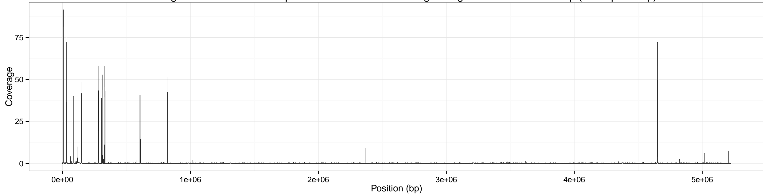
Coverage across cereus for input SRR1749070-0.05x using sliding window of size: 500 bp (overlap 250 bp)
