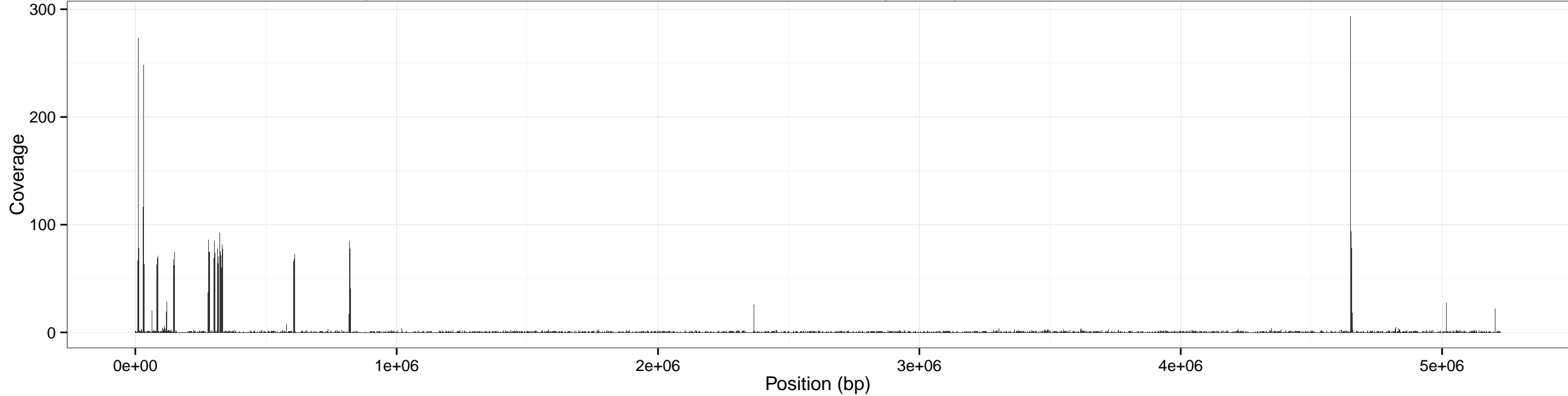
Coverage across cereus for input SRR1749070-0.05x using sliding window of size: 100 bp (overlap 50 bp)
