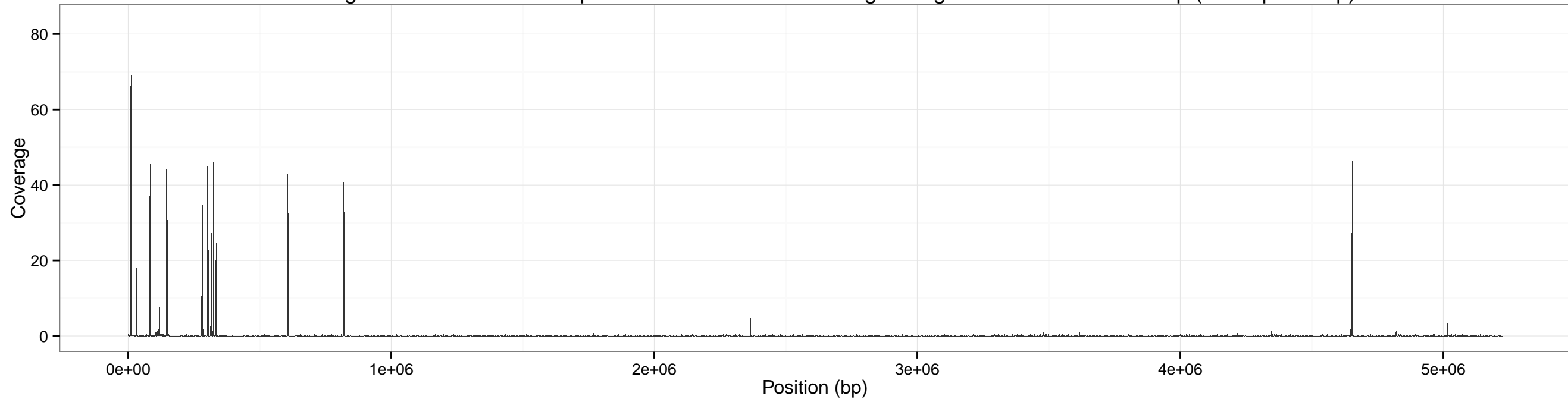
Coverage across cereus for input SRR1749070-0.05x using sliding window of size: 1000 bp (overlap 500 bp)
