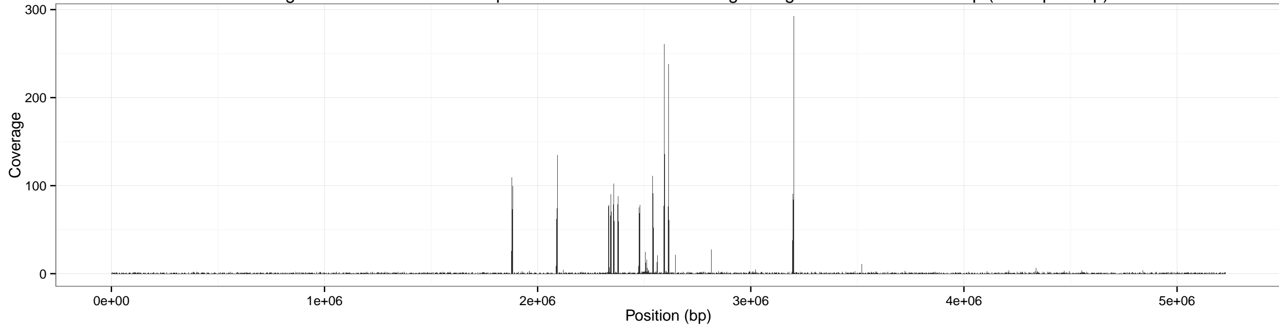
Coverage across anthracis for input SRR1749070-0.05x using sliding window of size: 100 bp (overlap 50 bp)
