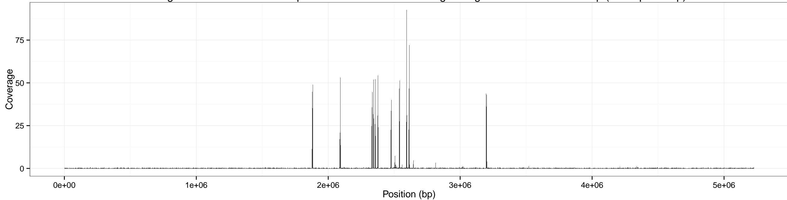
Coverage across anthracis for input SRR1749070-0.05x using sliding window of size: 1000 bp (overlap 500 bp)
