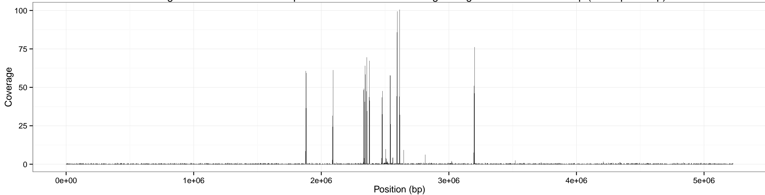
Coverage accross anthracis for input SRR1749070-0.05x using sliding window of size: 500 bp (overlap 250 bp)
