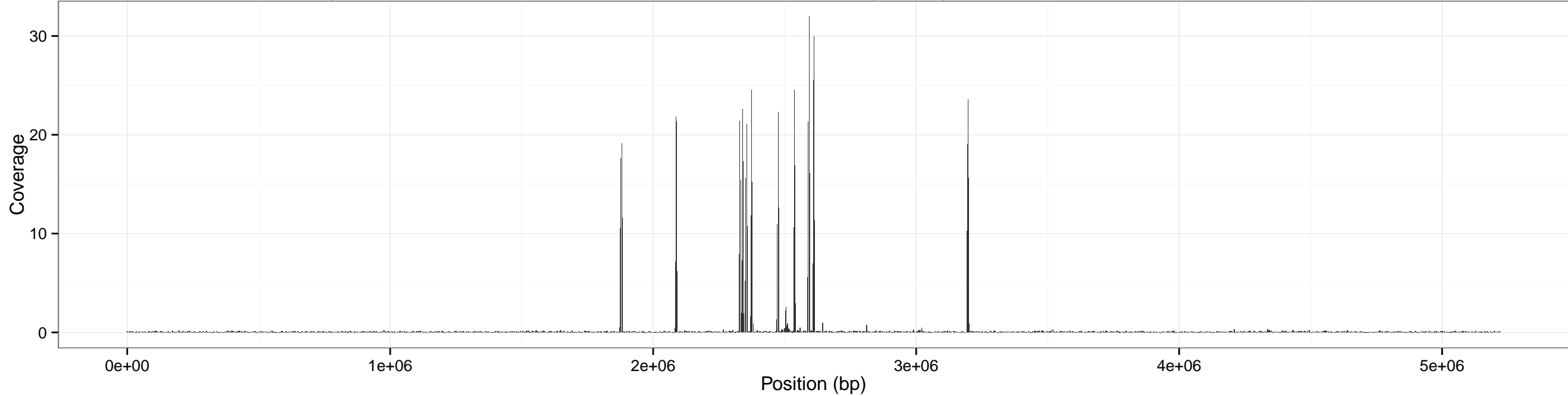
Coverage across anthracis for input SRR1749070-0.05x using sliding window of size: 5000 bp (overlap 2500 bp)
