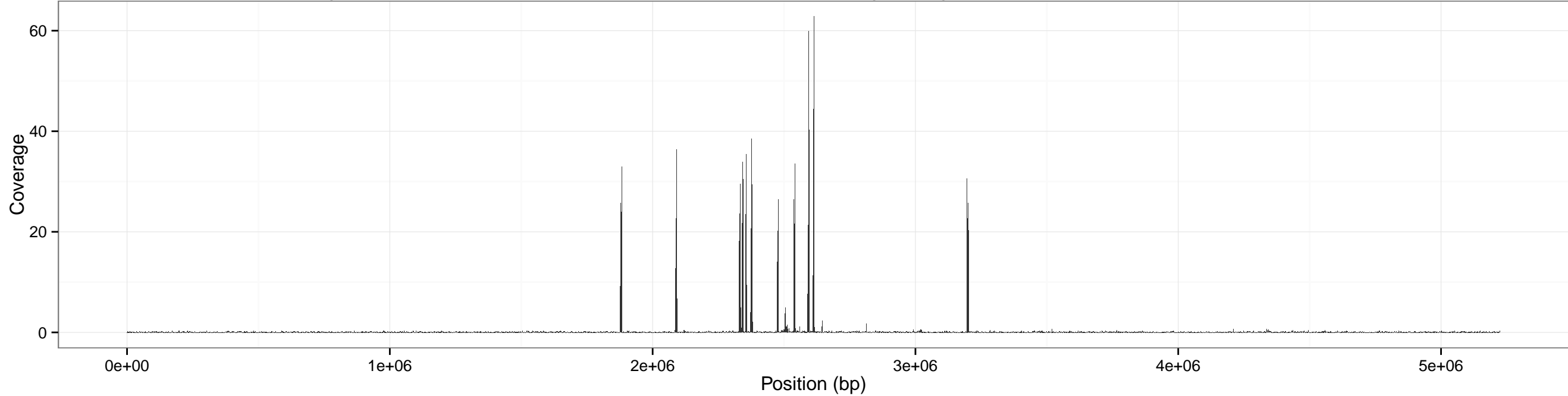
Coverage across anthracis for input SRR1749070-0.05x using sliding window of size: 2000 bp (overlap 1000 bp)
