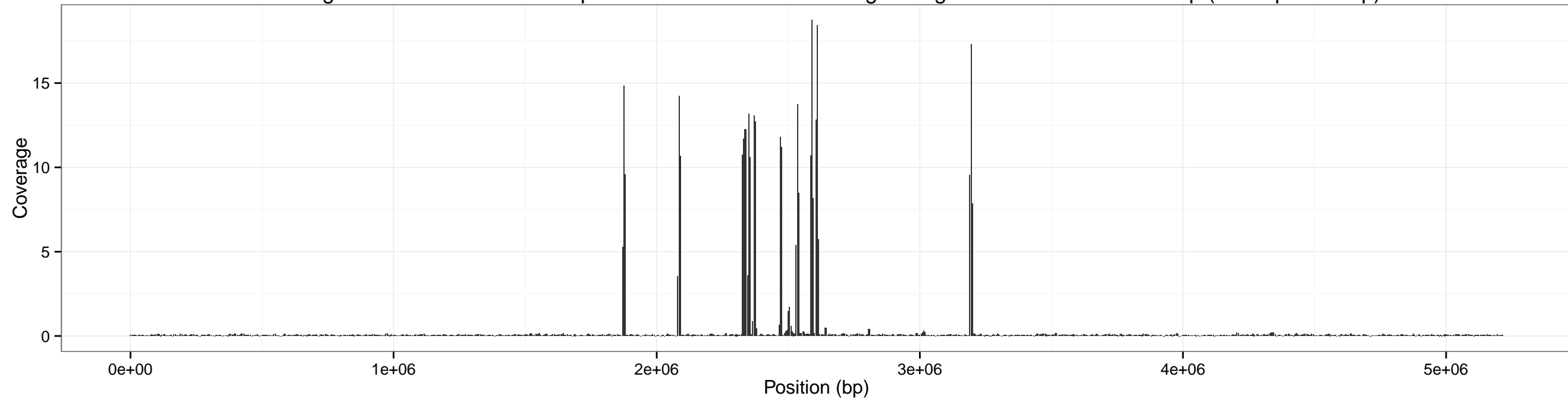
Coverage across anthracis for input SRR1749070-0.05x using sliding window of size: 10000 bp (overlap 5000 bp)
