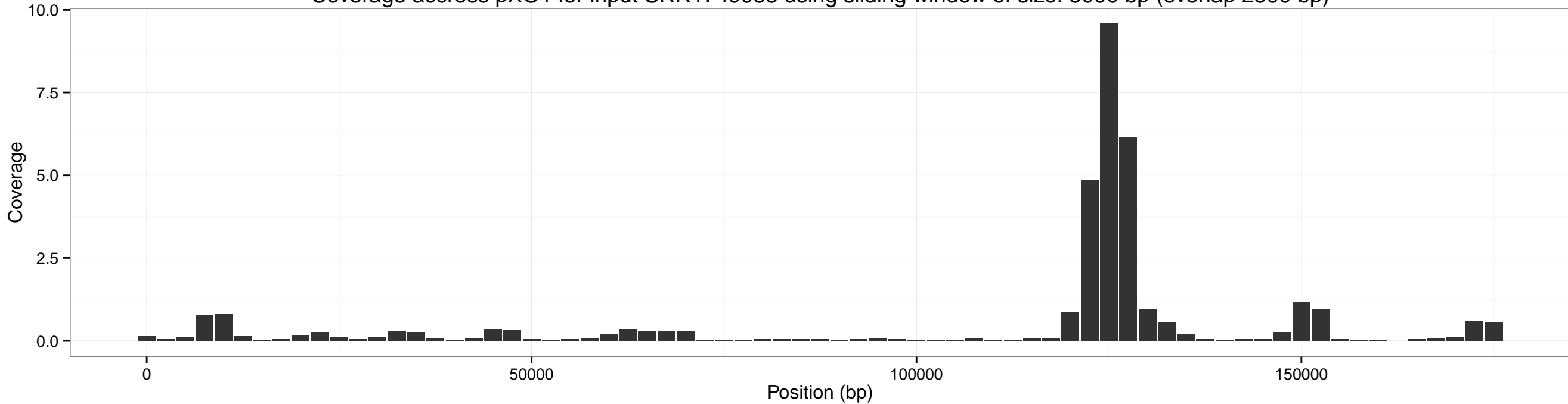
Coverage across pXO1 for input SRR1749083 using sliding window of size: 5000 bp (overlap 2500 bp)
