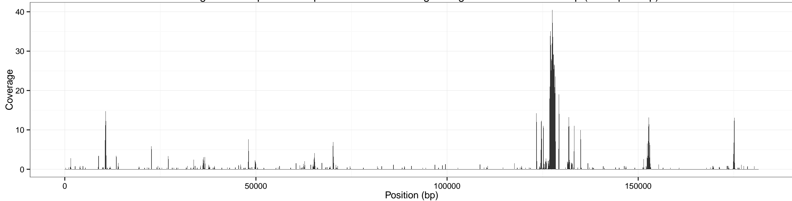
Coverage accross pXO1 for input SRR1749083 using sliding window of size: 100 bp (overlap 50 bp)
