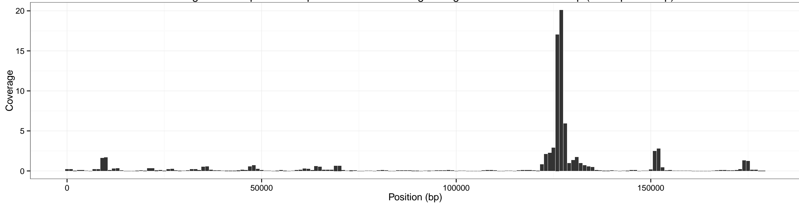
Coverage across pXO1 for input SRR1749083 using sliding window of size: 2000 bp (overlap 1000 bp)
