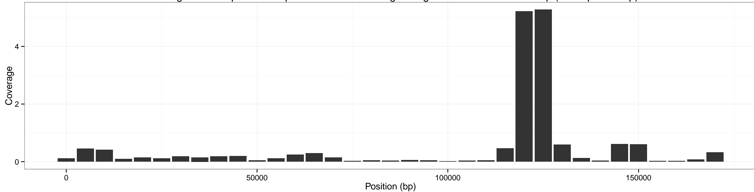
Coverage accross pXO1 for input SRR1749083 using sliding window of size: 10000 bp (overlap 5000 bp)
