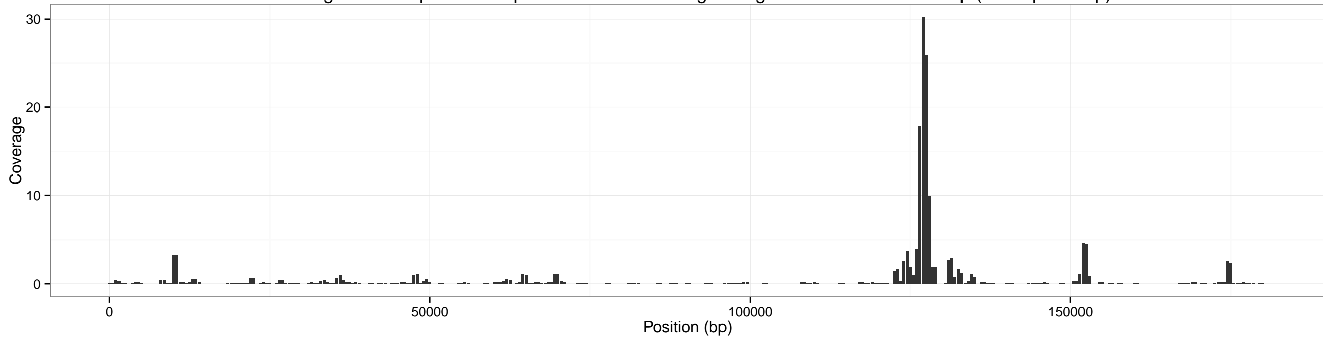
Coverage across pXO1 for input SRR1749083 using sliding window of size: 1000 bp (overlap 500 bp)
