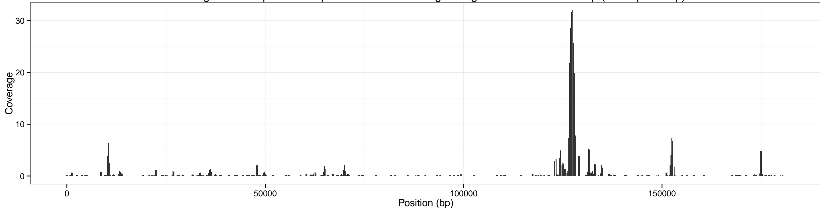
Coverage accross pXO1 for input SRR1749083 using sliding window of size: 500 bp (overlap 250 bp)
