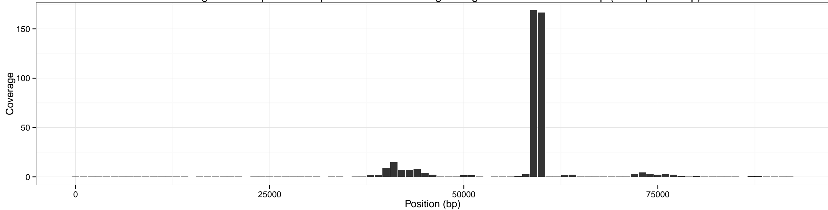
Coverage accross pXO2 for input SRR1748708 using sliding window of size: 2000 bp (overlap 1000 bp)
