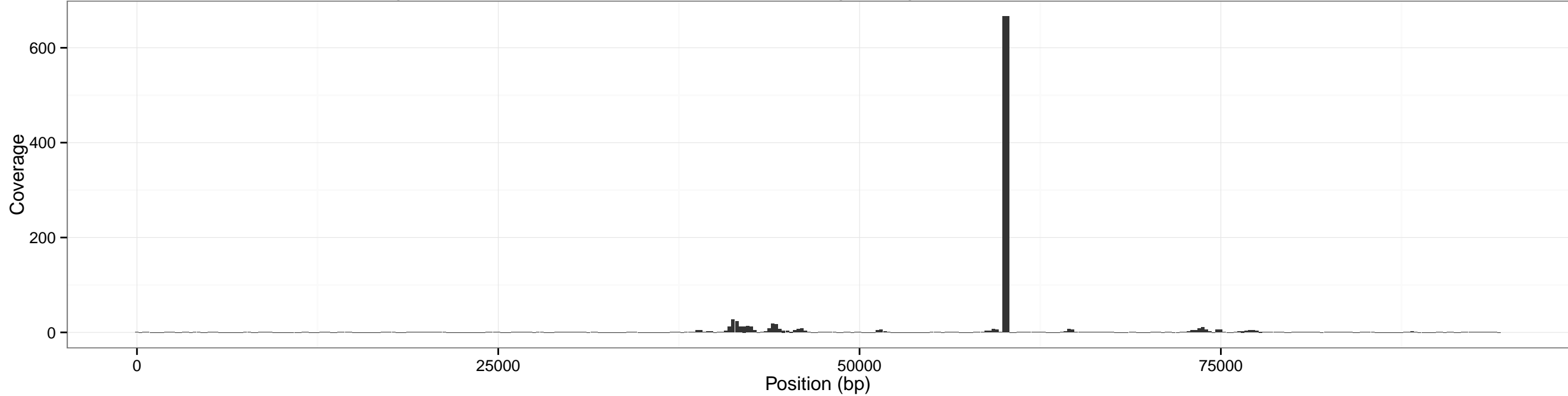
Coverage accross pXO2 for input SRR1748708 using sliding window of size: 500 bp (overlap 250 bp)
