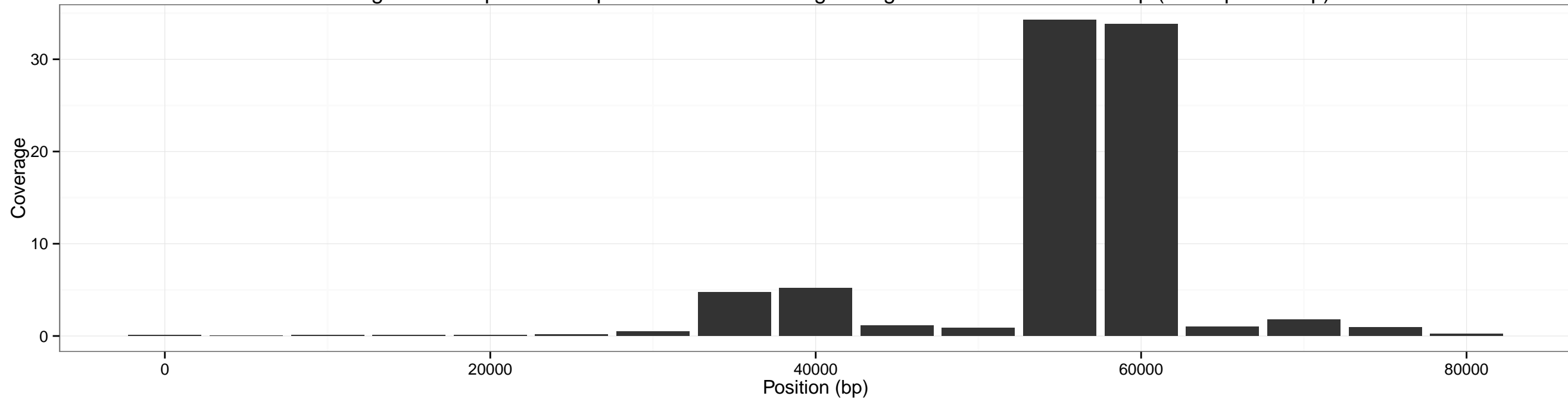
Coverage accross pXO2 for input SRR1748708 using sliding window of size: 10000 bp (overlap 5000 bp)
