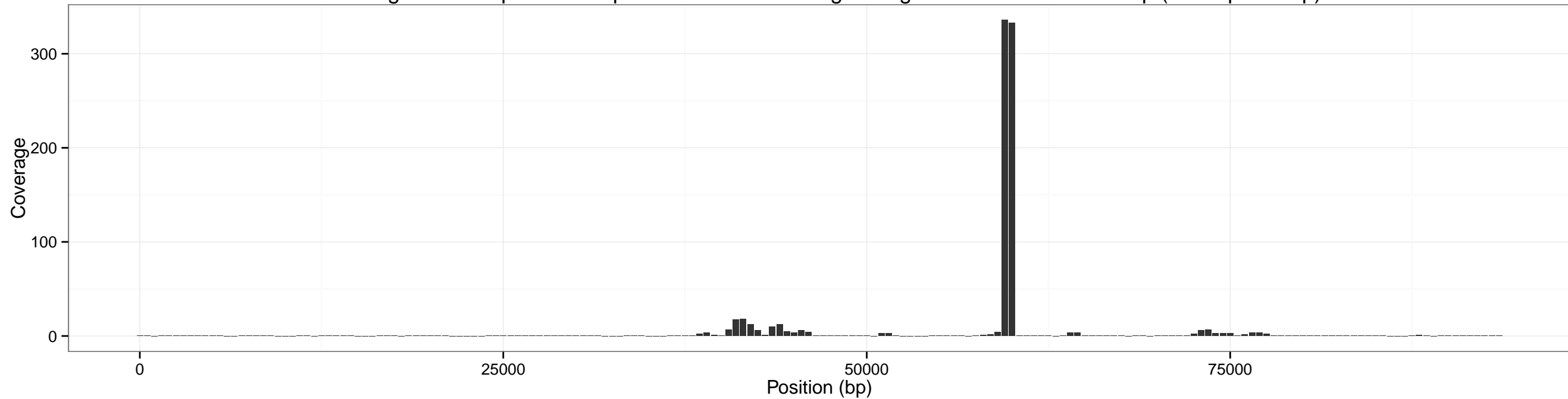
Coverage accross pXO2 for input SRR1748708 using sliding window of size: 1000 bp (overlap 500 bp)
