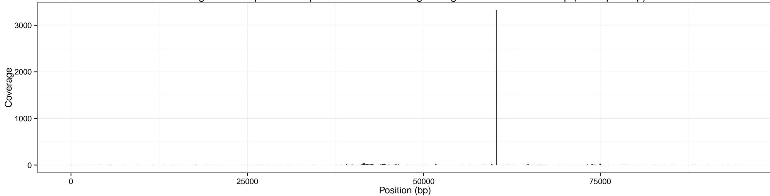
Coverage across pXO2 for input SRR1748708 using sliding window of size: 100 bp (overlap 50 bp)
