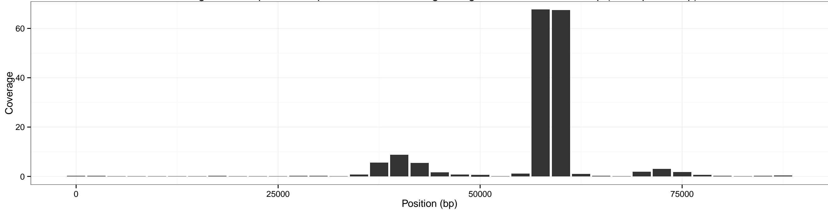
Coverage accross pXO2 for input SRR1748708 using sliding window of size: 5000 bp (overlap 2500 bp)
