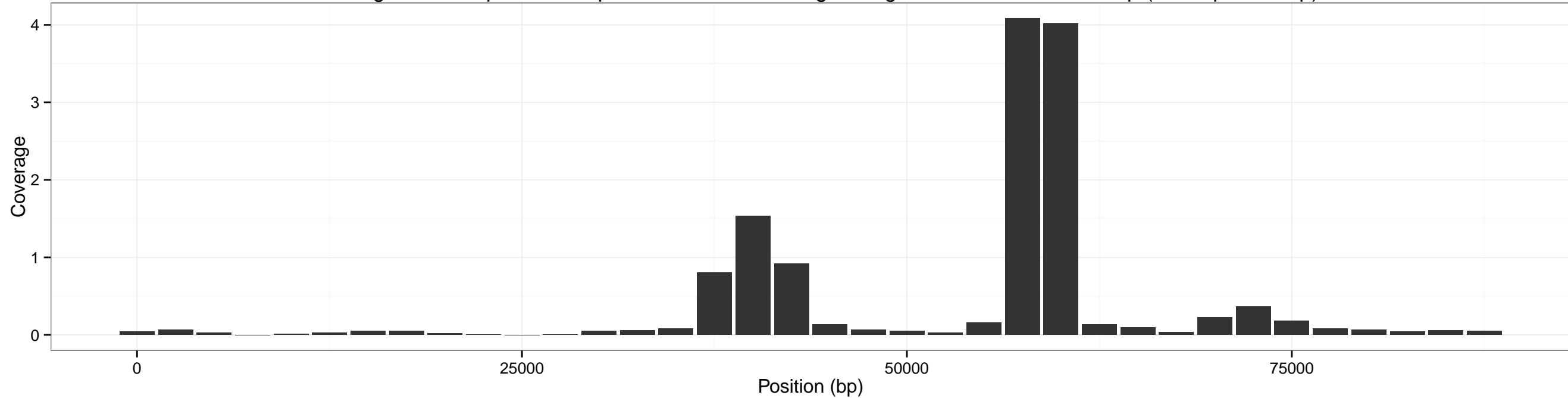
Coverage accross pXO2 for input SRR1748707 using sliding window of size: 5000 bp (overlap 2500 bp)
