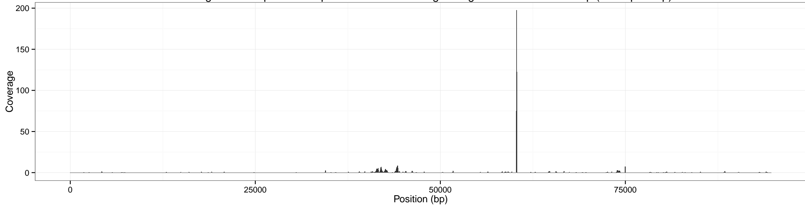
Coverage accross pXO2 for input SRR1748707 using sliding window of size: 100 bp (overlap 50 bp)
