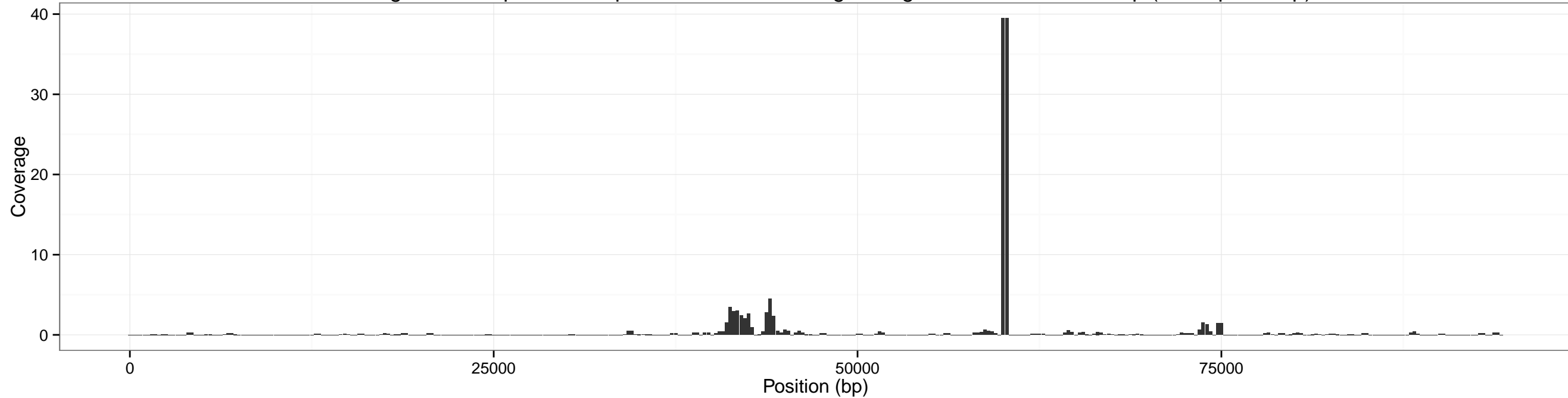
Coverage accross pXO2 for input SRR1748707 using sliding window of size: 500 bp (overlap 250 bp)
