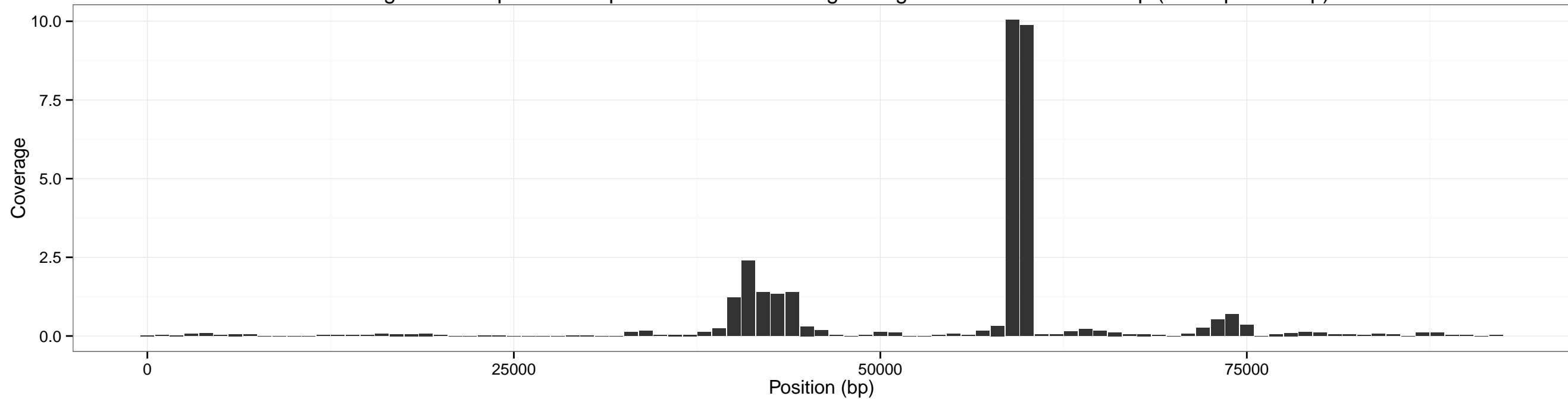
Coverage accross pXO2 for input SRR1748707 using sliding window of size: 2000 bp (overlap 1000 bp)
