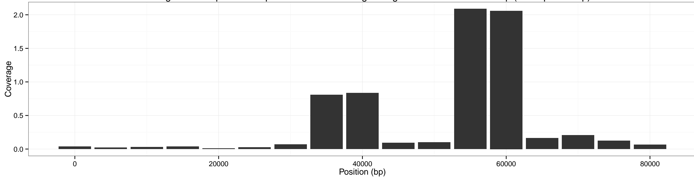
Coverage accross pXO2 for input SRR1748707 using sliding window of size: 10000 bp (overlap 5000 bp)
