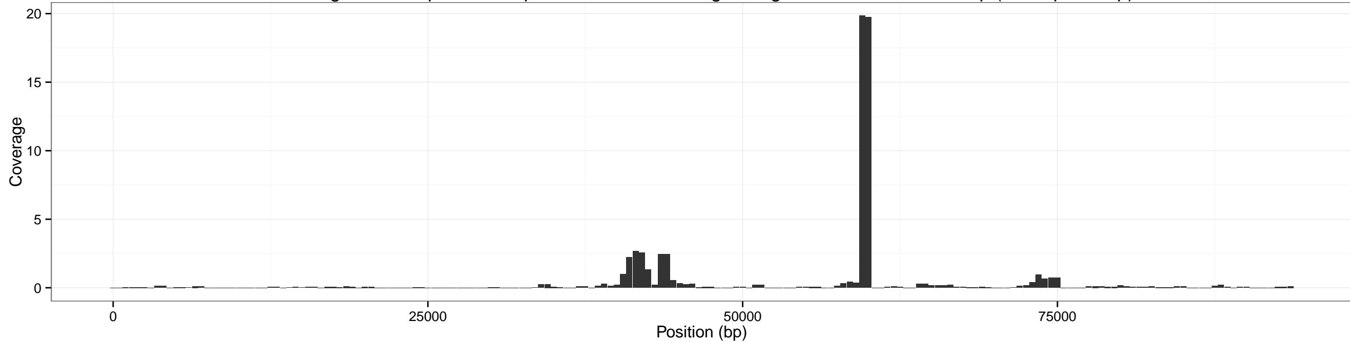
Coverage across pXO2 for input SRR1748707 using sliding window of size: 1000 bp (overlap 500 bp)
