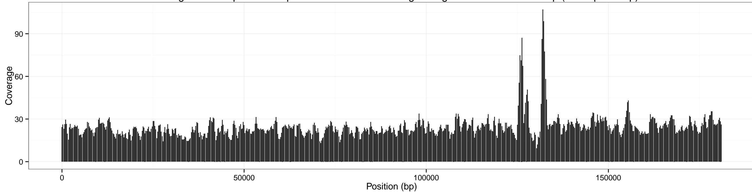
Coverage accross pXO1 for input SRR1749070-5x using sliding window of size: 500 bp (overlap 250 bp)
