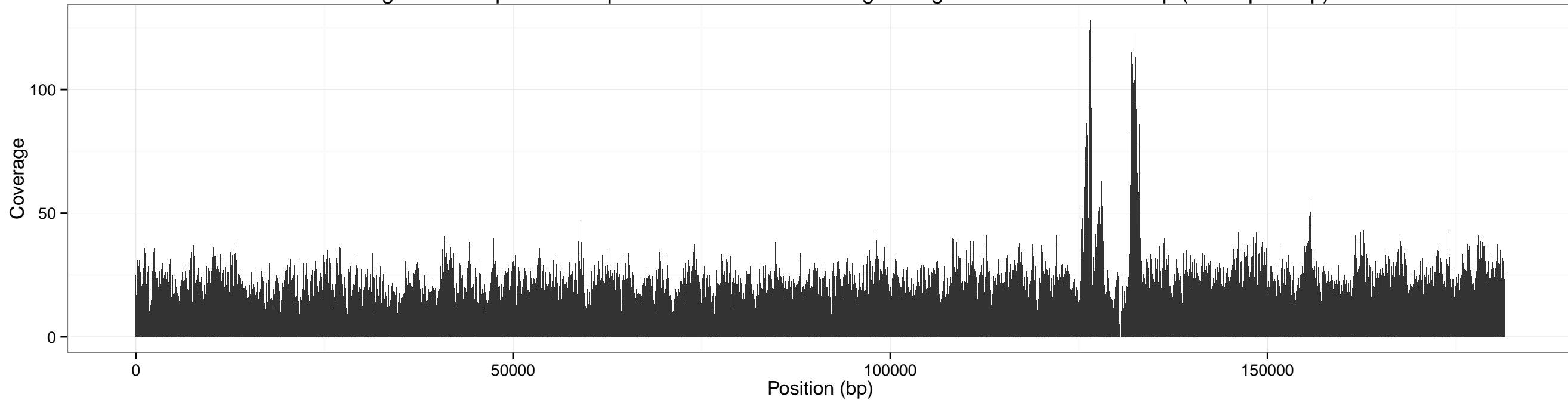
Coverage accross pXO1 for input SRR1749070-5x using sliding window of size: 100 bp (overlap 50 bp)
