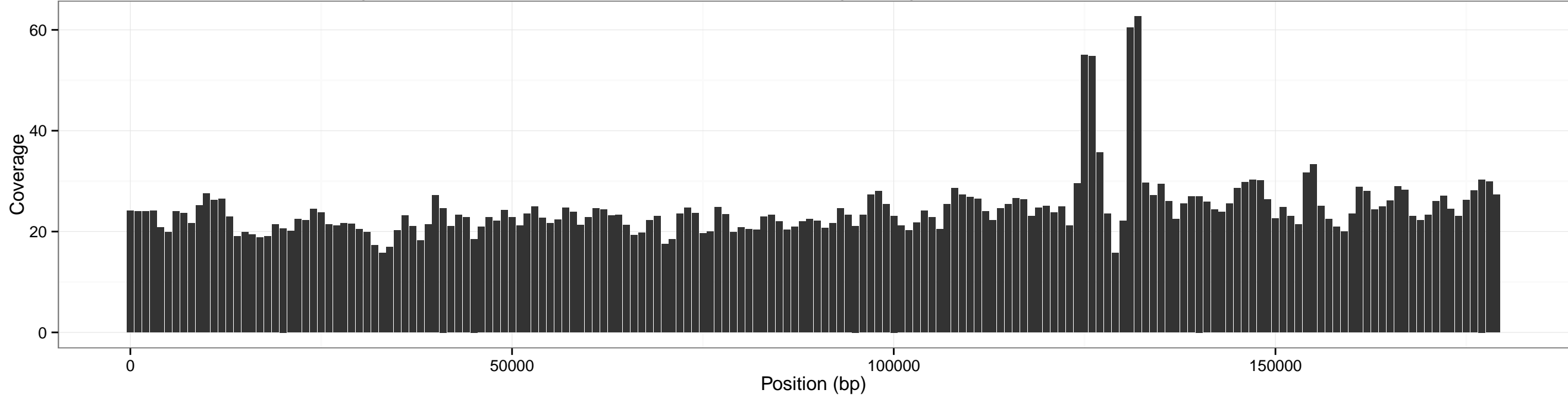
Coverage accross pXO1 for input SRR1749070-5x using sliding window of size: 2000 bp (overlap 1000 bp)
