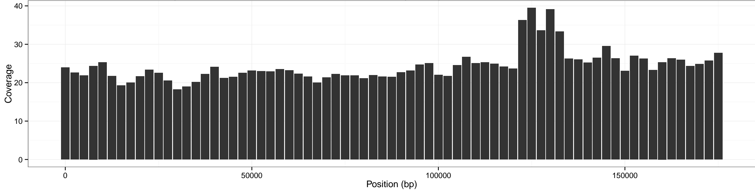
Coverage accross pXO1 for input SRR1749070-5x using sliding window of size: 5000 bp (overlap 2500 bp)
