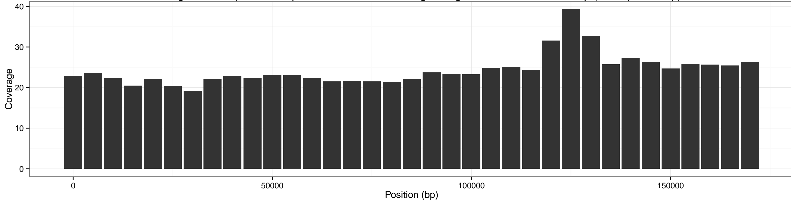
Coverage accross pXO1 for input SRR1749070-5x using sliding window of size: 10000 bp (overlap 5000 bp)
