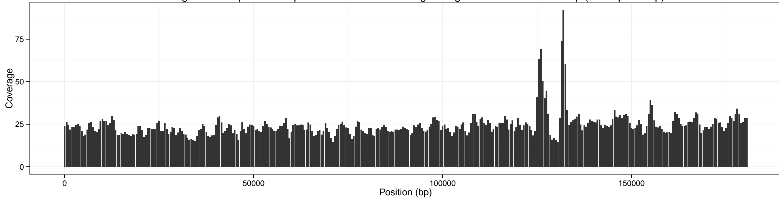
Coverage accross pXO1 for input SRR1749070-5x using sliding window of size: 1000 bp (overlap 500 bp)
