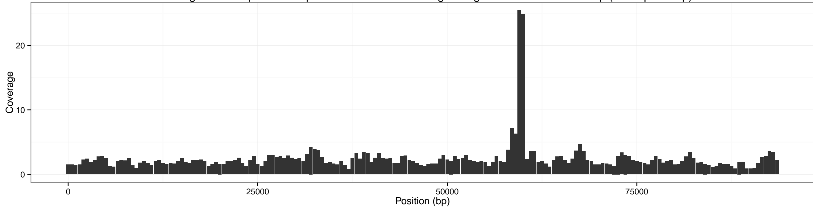
Coverage accross pXO2 for input SRR1749070-1x using sliding window of size: 1000 bp (overlap 500 bp)
