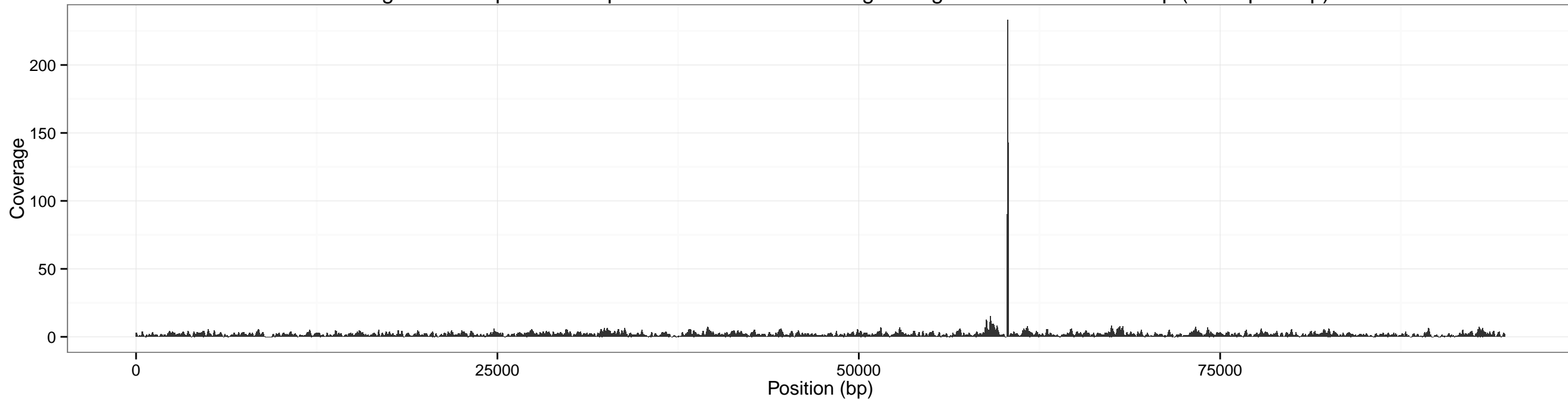
Coverage across pXO2 for input SRR1749070-1x using sliding window of size: 100 bp (overlap 50 bp)
