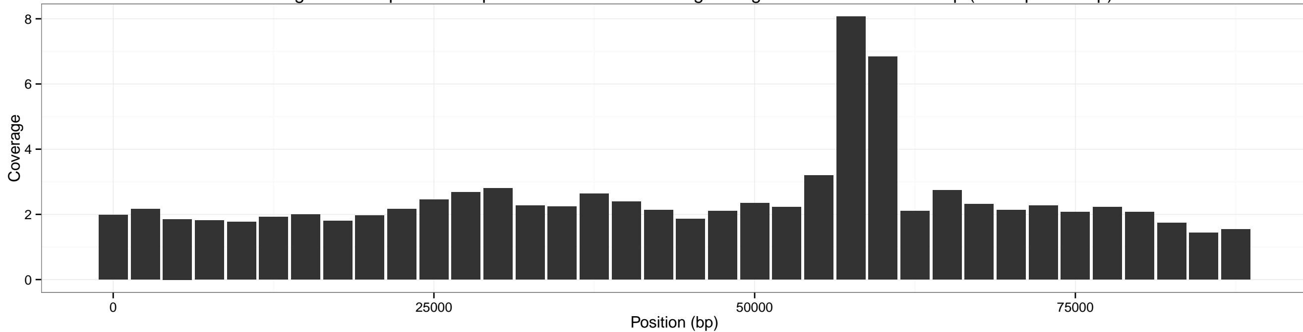
Coverage accross pXO2 for input SRR1749070-1x using sliding window of size: 5000 bp (overlap 2500 bp)
