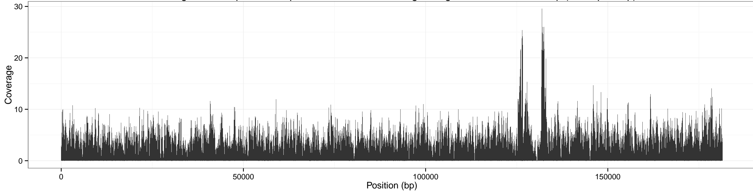
Coverage across pXO1 for input SRR1749070-1x using sliding window of size: 100 bp (overlap 50 bp)
