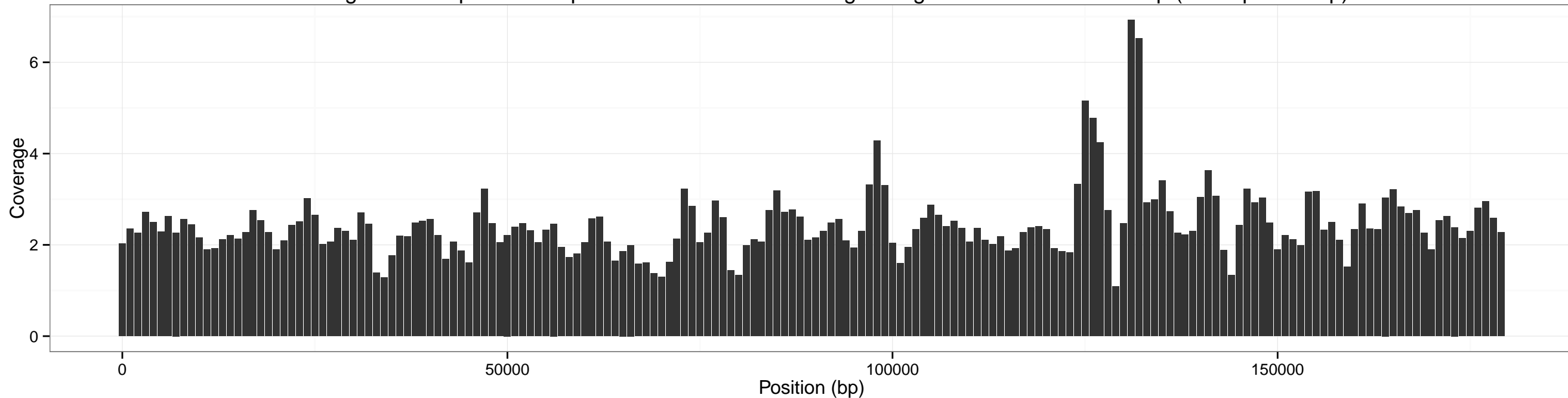
Coverage across pXO1 for input SRR1749070-0.5x using sliding window of size: 2000 bp (overlap 1000 bp)
