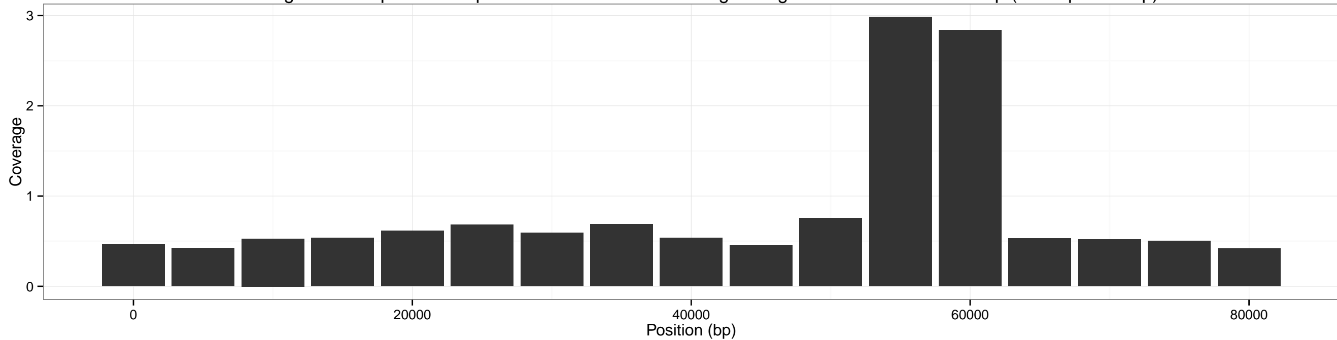
Coverage accross pXO2 for input SRR1749070-0.25x using sliding window of size: 10000 bp (overlap 5000 bp)
