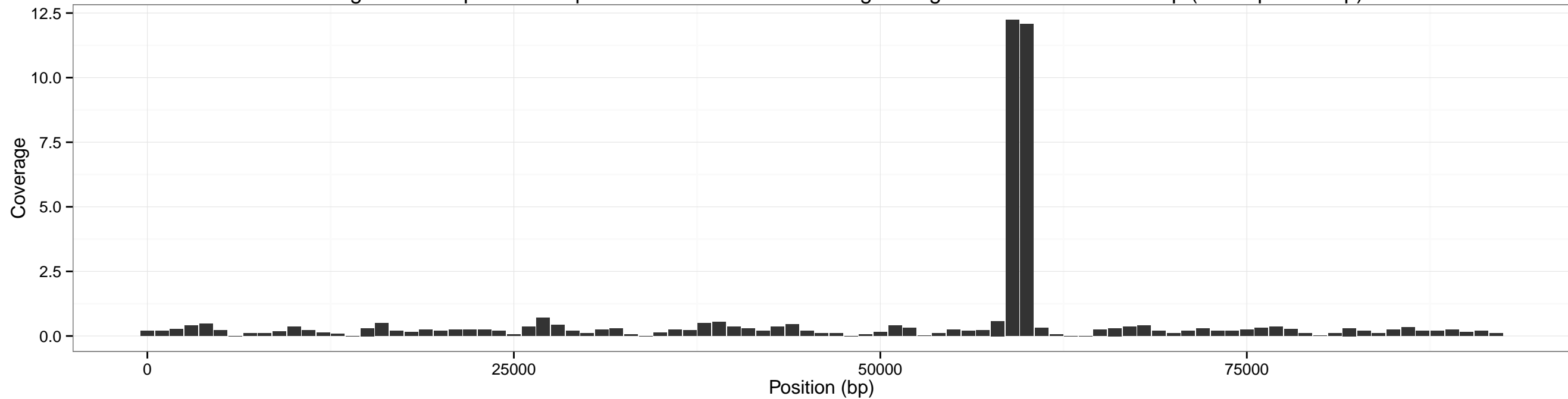
Coverage accross pXO2 for input SRR1749070-0.10x using sliding window of size: 2000 bp (overlap 1000 bp)
