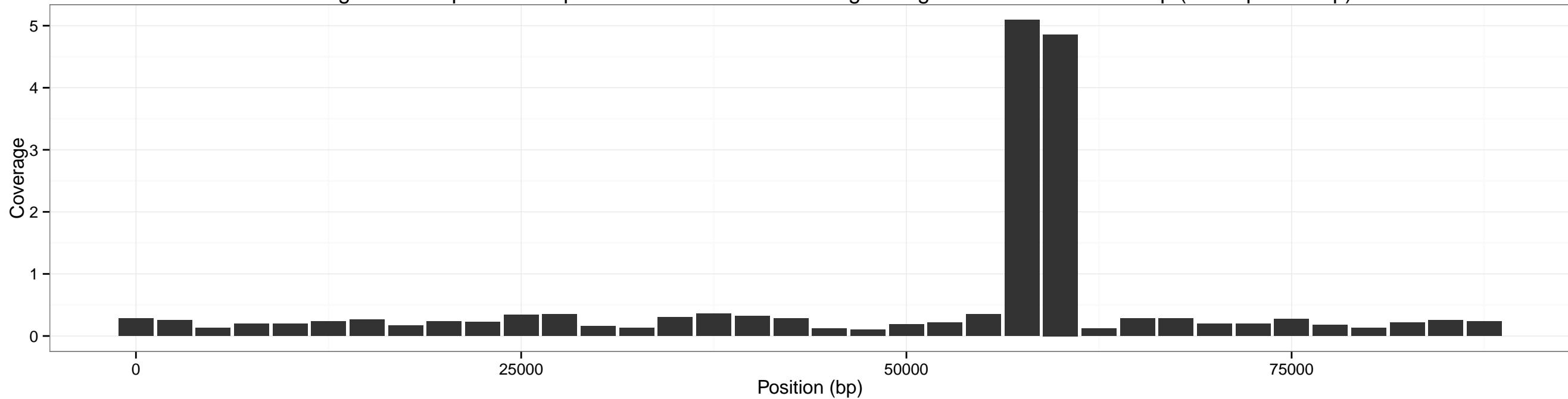
Coverage across pXO2 for input SRR1749070-0.10x using sliding window of size: 5000 bp (overlap 2500 bp)
