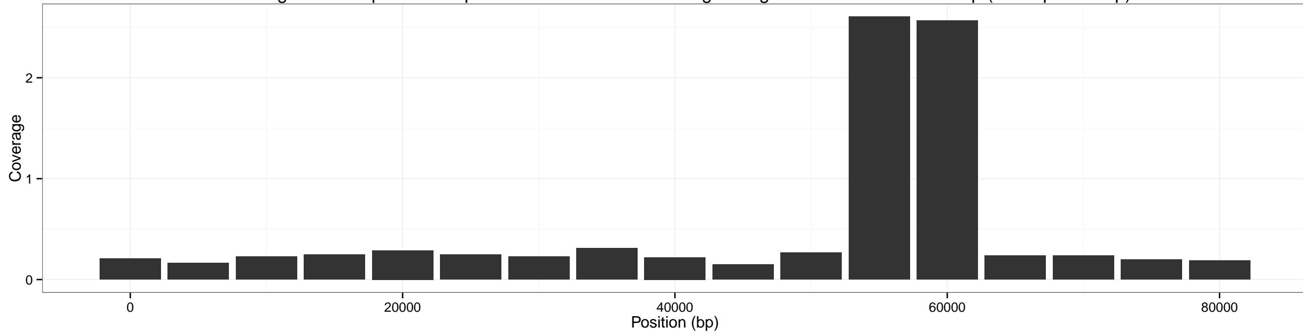
Coverage across pXO2 for input SRR1749070-0.10x using sliding window of size: 10000 bp (overlap 5000 bp)
