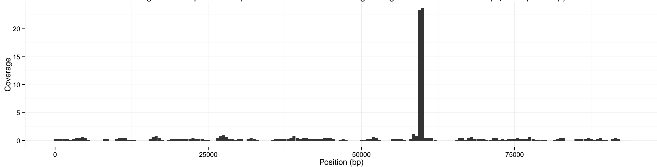
Coverage accross pXO2 for input SRR1749070-0.10x using sliding window of size: 1000 bp (overlap 500 bp)
