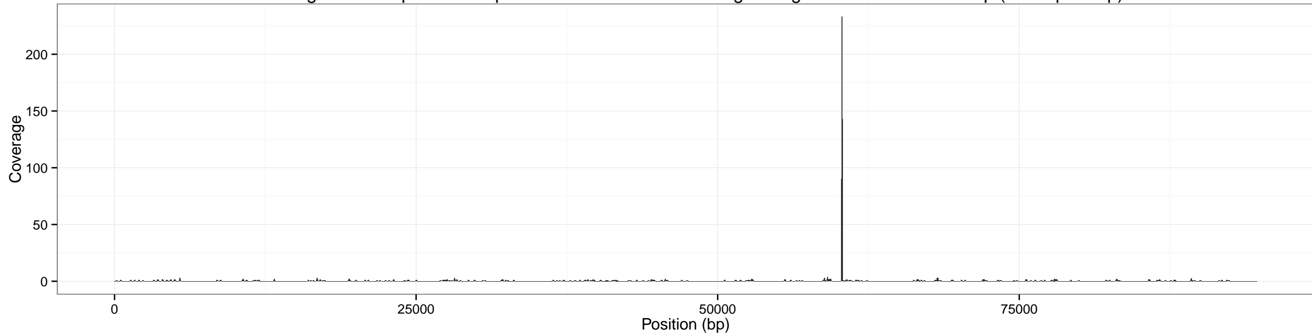
Coverage accross pXO2 for input SRR1749070-0.10x using sliding window of size: 100 bp (overlap 50 bp)
