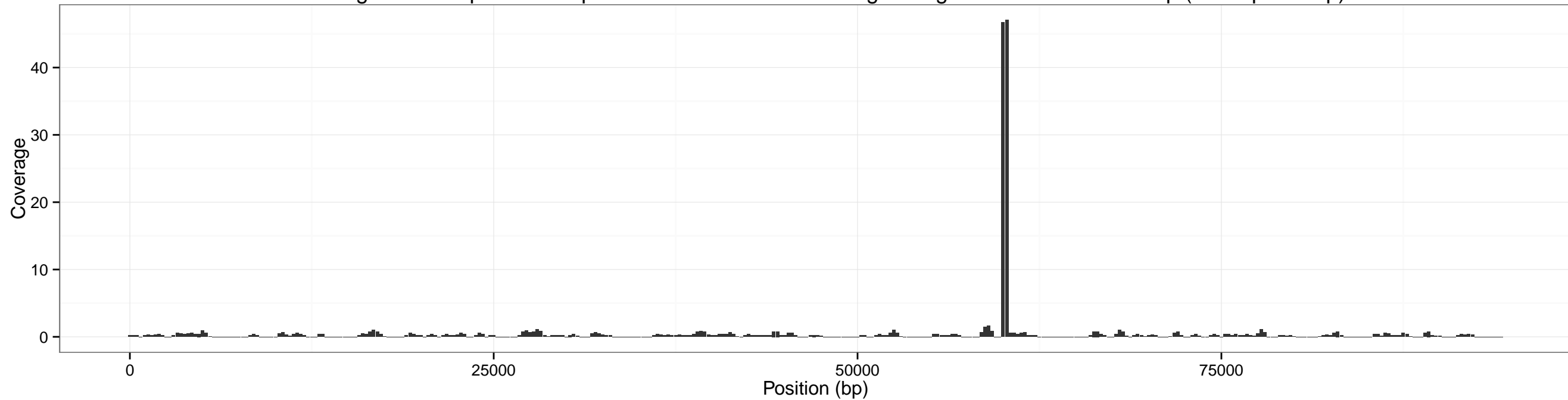
Coverage accross pXO2 for input SRR1749070-0.10x using sliding window of size: 500 bp (overlap 250 bp)
