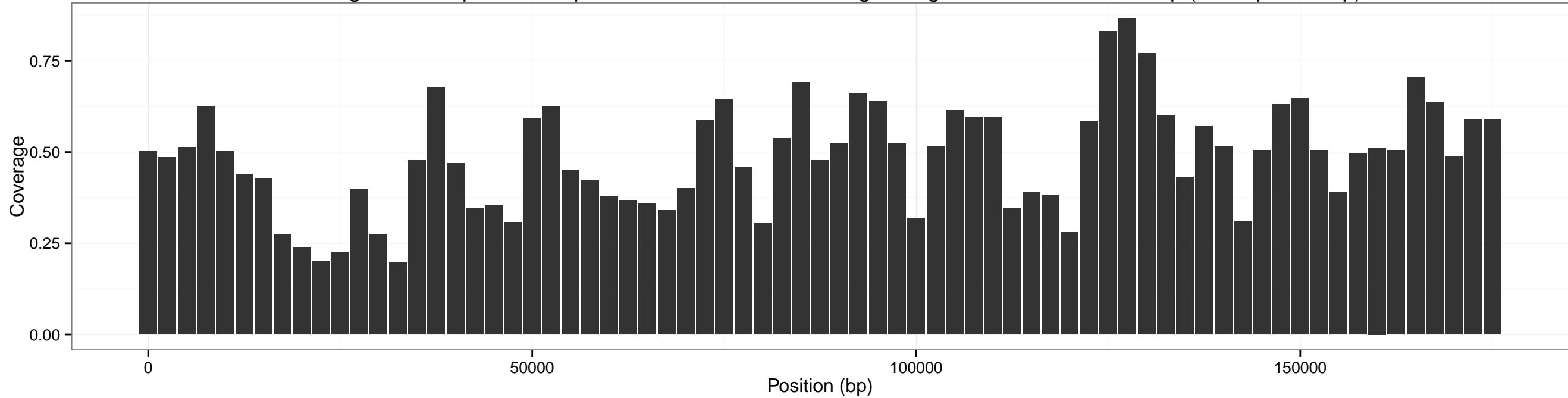
Coverage accross pXO1 for input SRR1749070-0.10x using sliding window of size: 5000 bp (overlap 2500 bp)
