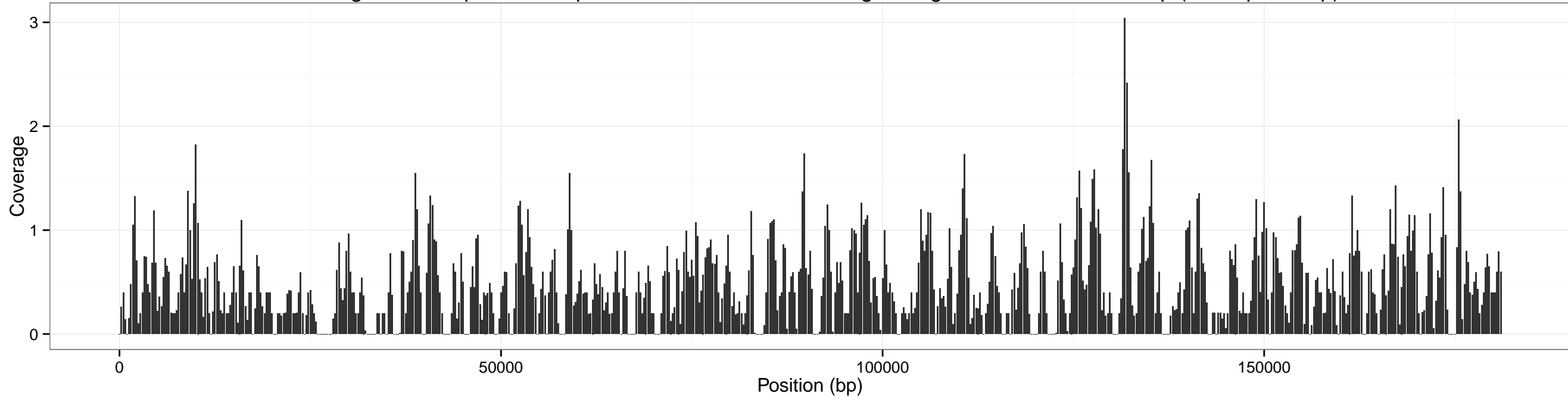
Coverage across pXO1 for input SRR1749070-0.10x using sliding window of size: 500 bp (overlap 250 bp)
