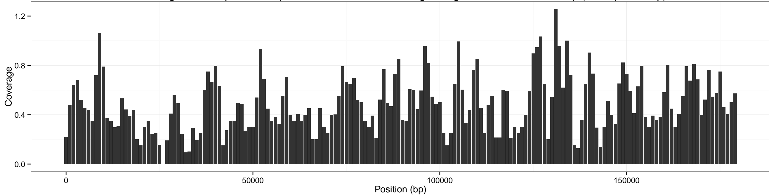
Coverage across pXO1 for input SRR1749070-0.10x using sliding window of size: 2000 bp (overlap 1000 bp)
