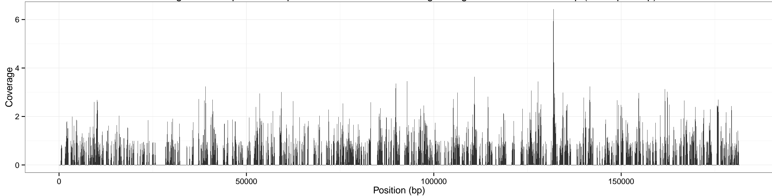
Coverage accross pXO1 for input SRR1749070-0.10x using sliding window of size: 100 bp (overlap 50 bp)
