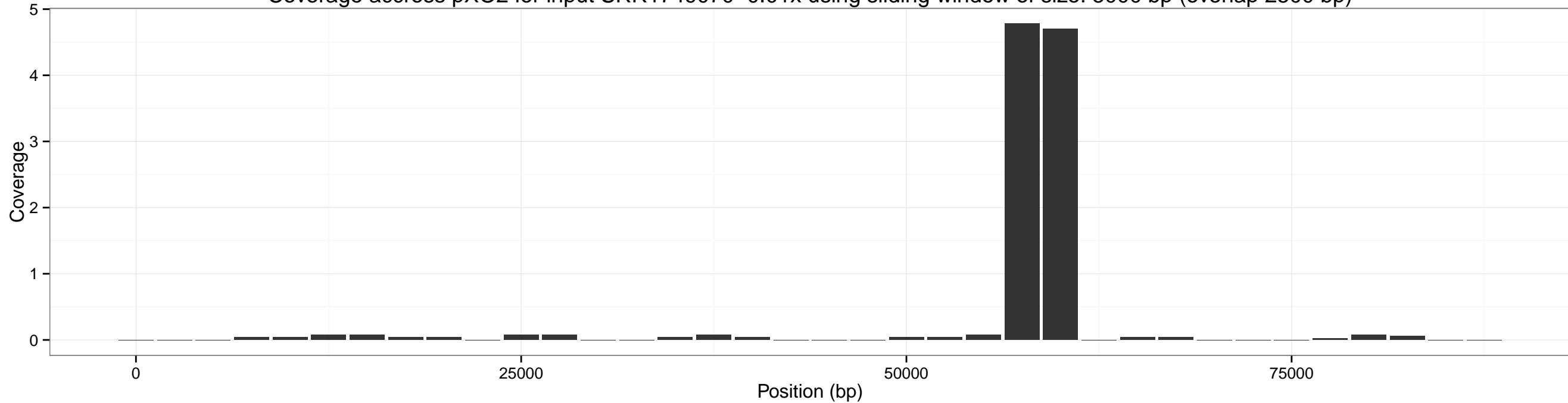
Coverage accross pXO2 for input SRR1749070-0.01x using sliding window of size: 5000 bp (overlap 2500 bp)
