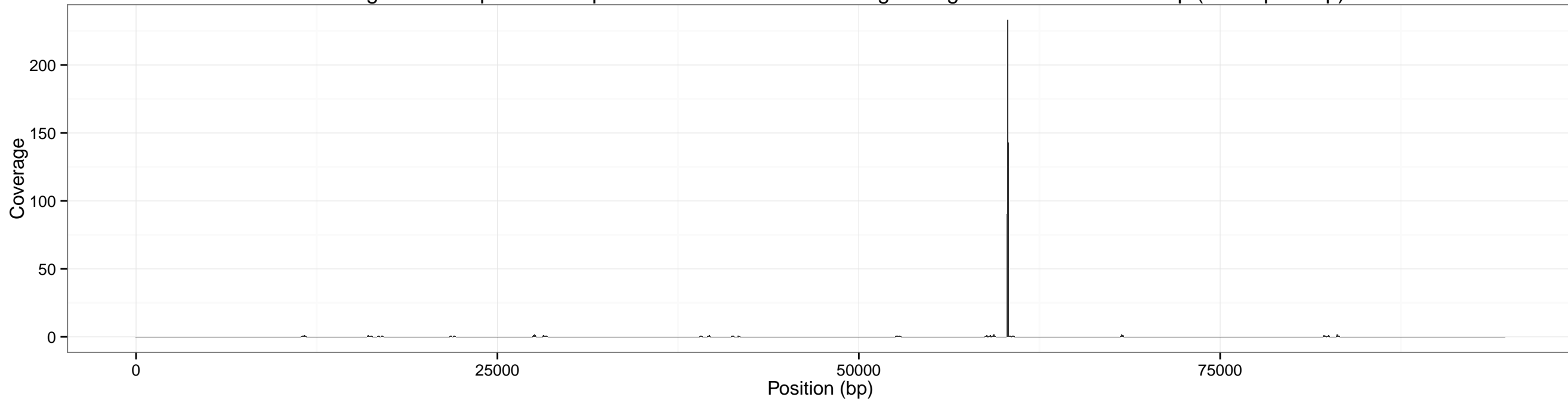
Coverage accross pXO2 for input SRR1749070-0.01x using sliding window of size: 100 bp (overlap 50 bp)
