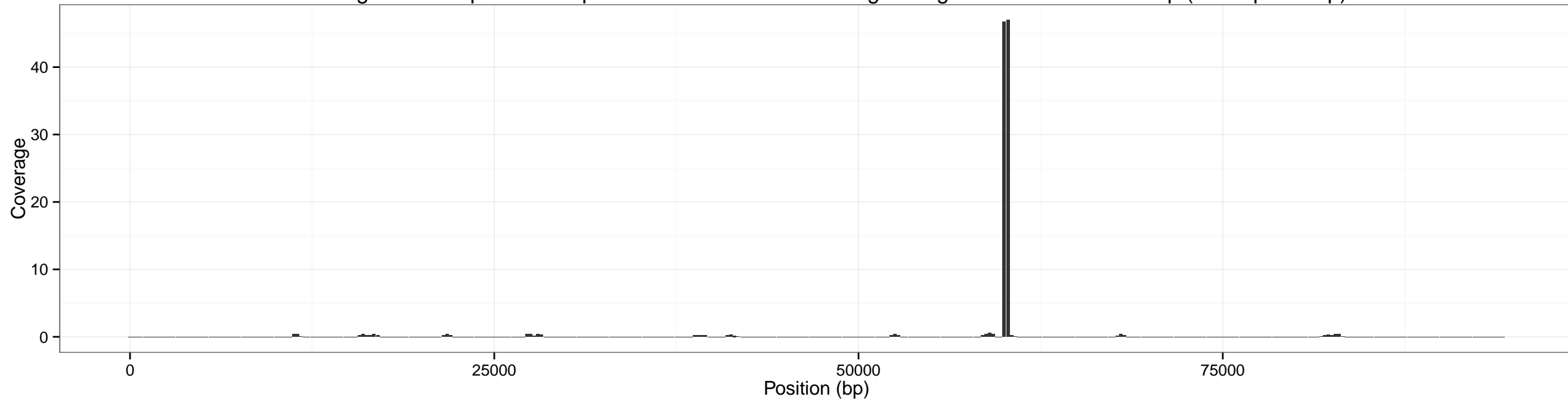
Coverage accross pXO2 for input SRR1749070-0.01x using sliding window of size: 500 bp (overlap 250 bp)
