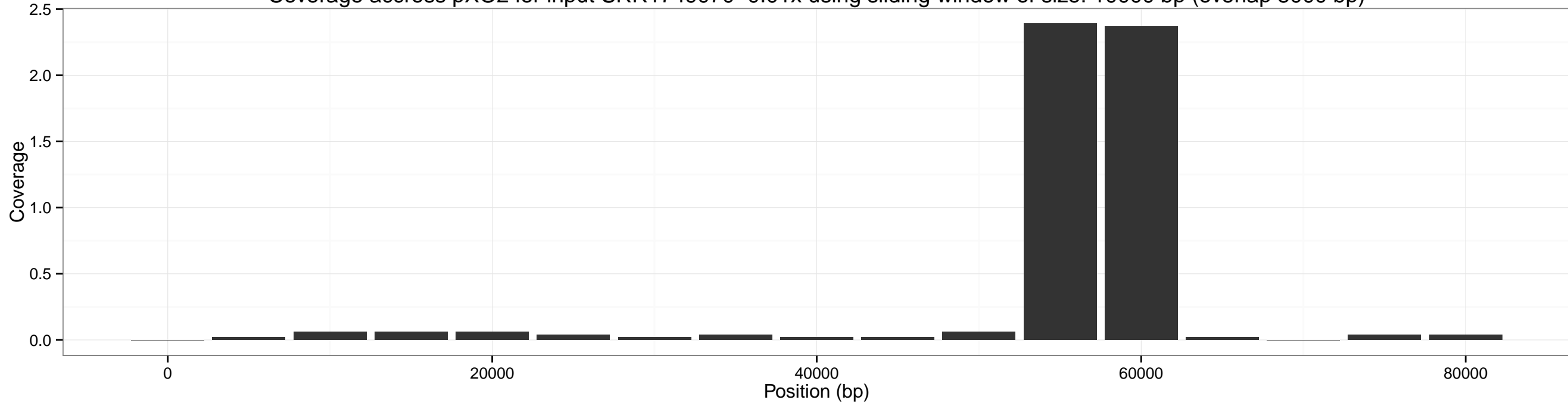
Coverage accross pXO2 for input SRR1749070-0.01x using sliding window of size: 10000 bp (overlap 5000 bp)
