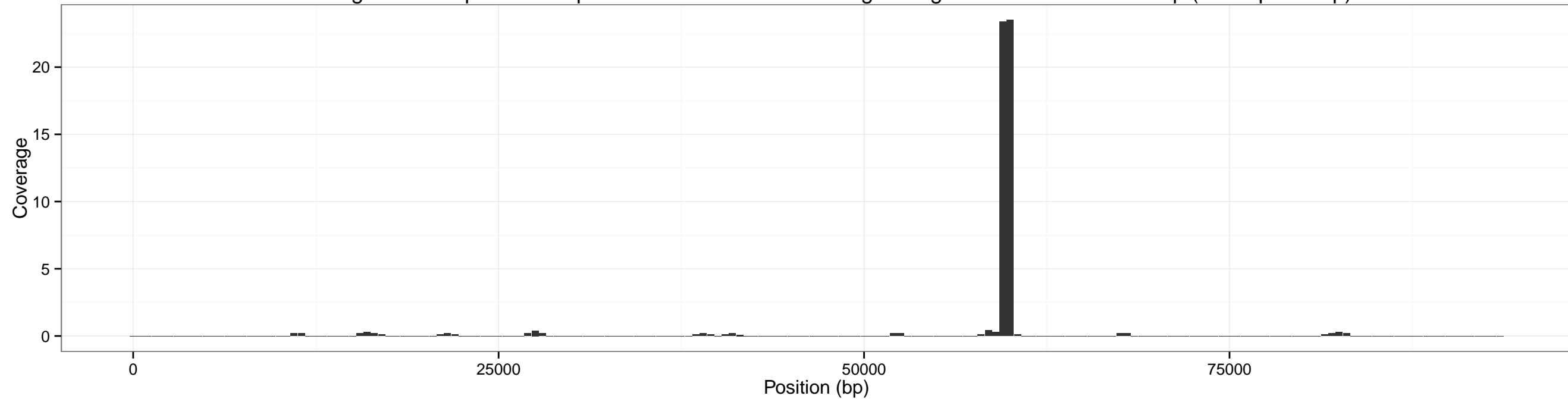
Coverage accross pXO2 for input SRR1749070-0.01x using sliding window of size: 1000 bp (overlap 500 bp)
