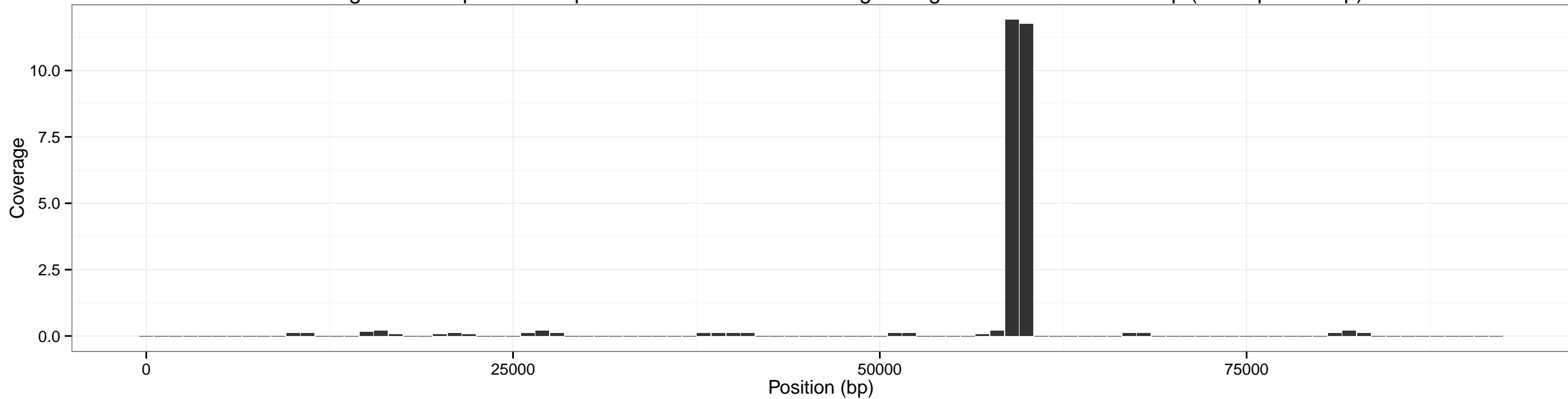
Coverage accross pXO2 for input SRR1749070-0.01x using sliding window of size: 2000 bp (overlap 1000 bp)
